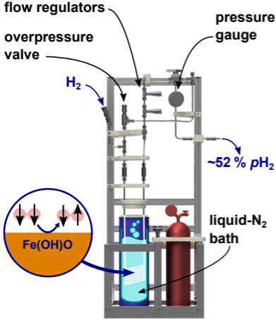
photo of assembled generator
