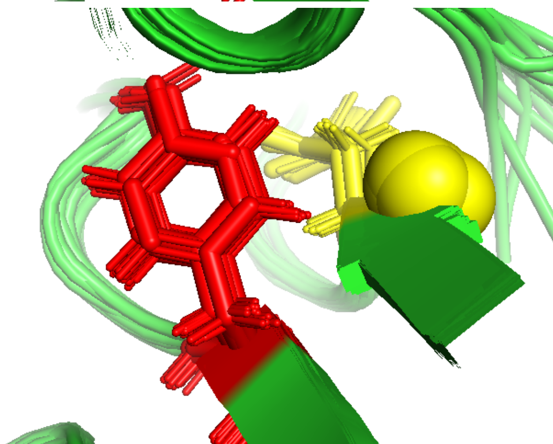
(b) 2NCL D28-Y37 (Ensemble)
