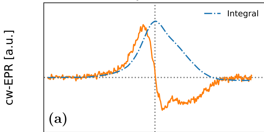
10-Doxyl-PC in DOPC
