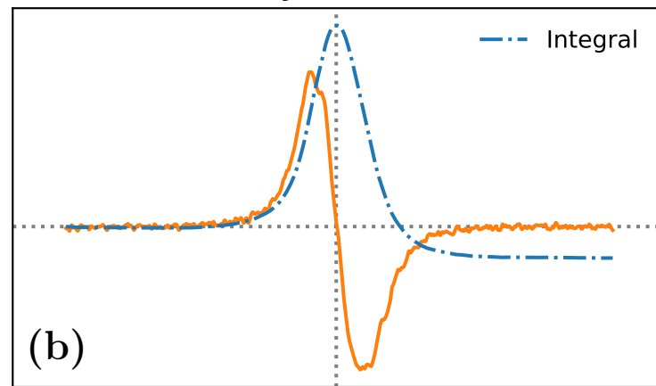
16-Doxyl-PC in DOPC
