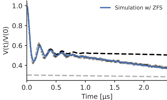
(c) TPP-AA 5 -NO • , Q-band
