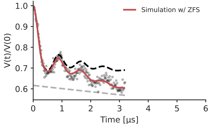
(b) TPP-AA 10 -NO • , X-band
