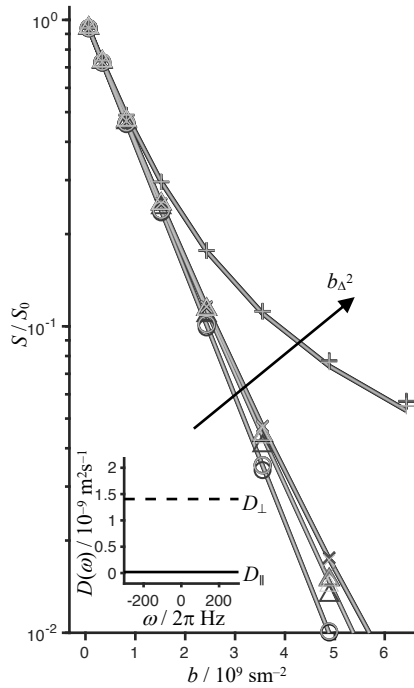
(b) lamellar liquid crystal at 291 K anisotropic Gaussian
