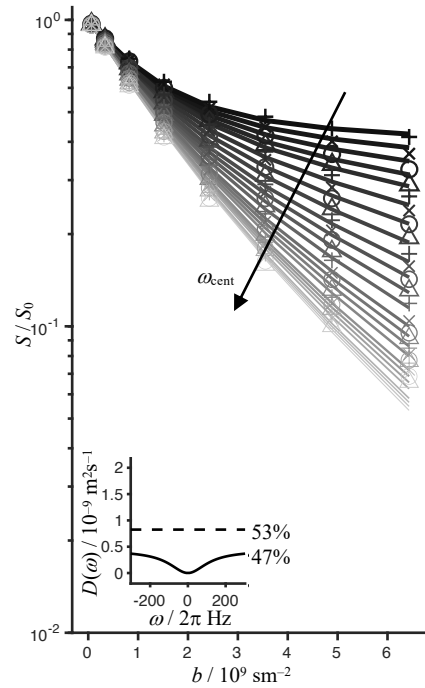
(c) yeast cell sediment at 278 K isotropic restricted + Gaussian
