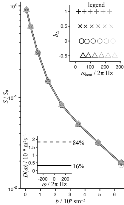
(a) water + brine at 291 K isotropic Gaussian fast + slow
