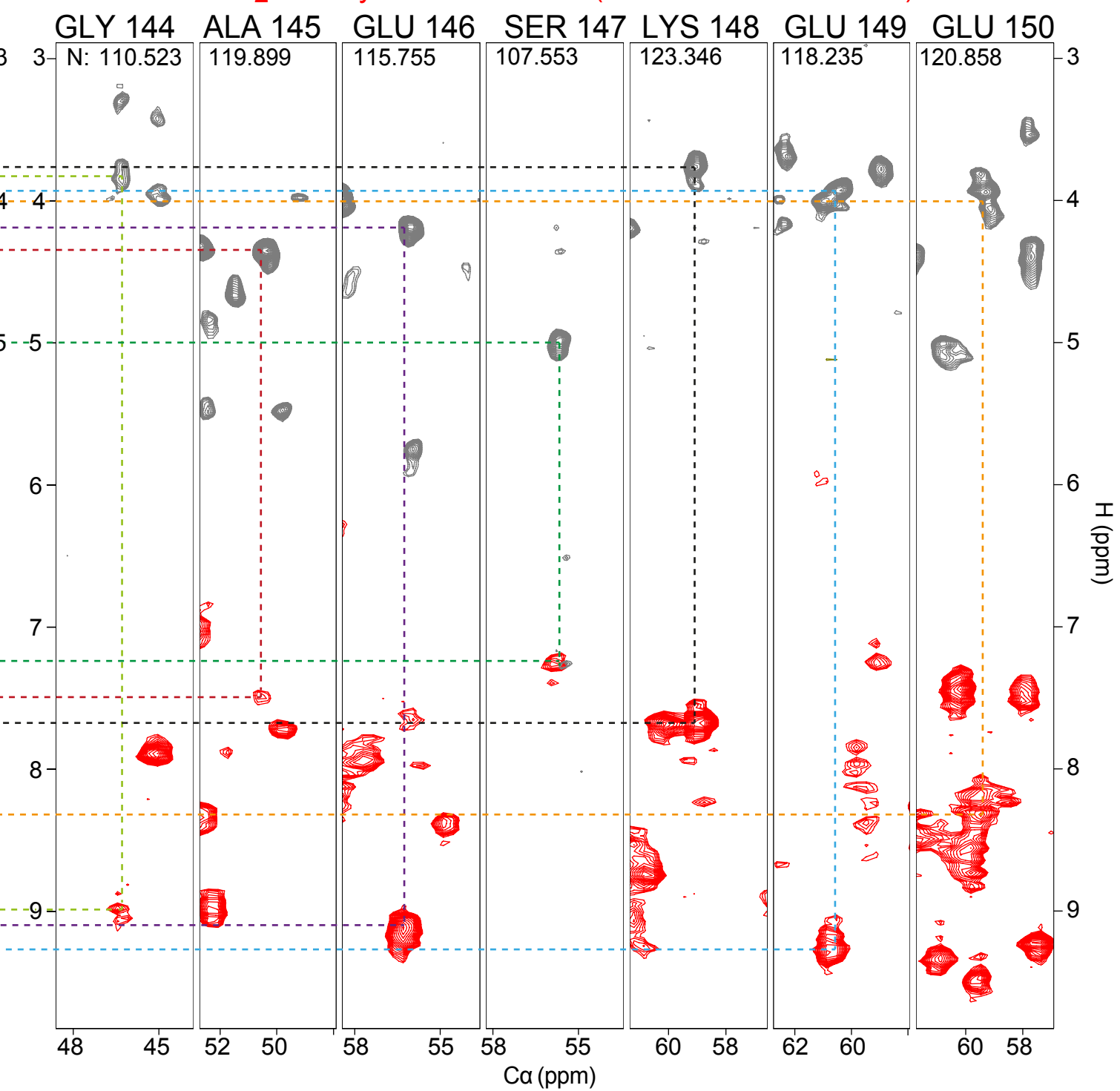
(b) 3D hNCαH H 2 O/M9/lysate-deuterated (600 MHz - 55 kHz MAS)
