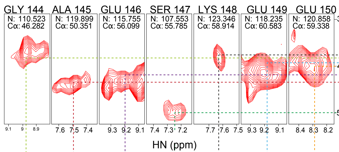
(a) 4D HaCaNH H 2 O/M9/lysate-deuterated (600 MHz - 55 kHz MAS)
