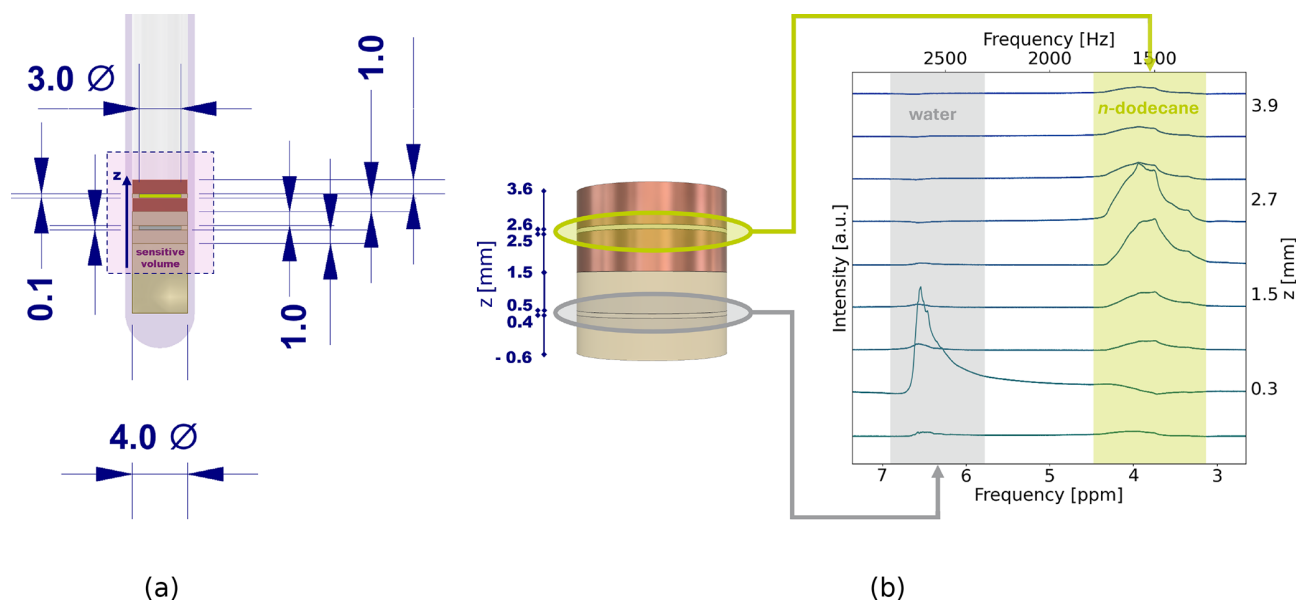
Figure 1. Sectional side view of experimental setup inside a shortened standard 5 mm NMR tube with cell dimensions given in mm (a) and 3D illustration of the setup with a spatially encoded chemical shift imaging of \text{H}_2\text{O} and n -dodecane in between the double coins (b). The cavities each have a diameter of 3 mm and a height of 0.1 mm. The coins each have a diameter of 4 mm and a height of 1 mm. The NMR-sensitive volume for homogeneous excitation is marked by a pink rectangle with dashed line and extends \pm 4 mm in the z direction from the center of the model setup. The spatial position of the liquids can be differentiated on a scale of about half a mm.
