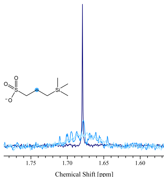
Figure 4. Line-narrowing and decoupling by monochromatic SSL applied to the central \text{CH}_2 multiplet (blue circle) of 200 \mu\text{M} DSS in \text{D}_2\text{O} . Blue line (scaled \times 2 ): Conventional 1D multiplet with an overall width of ca. 40 Hz and \Delta\nu = 2 Hz for the central line. Light blue (scaled \times 2 ): Broadened by deliberately miss-setting a shim current to an overall width of ca. 50 Hz. Dark blue line: The broadened spectrum was line narrowed and decoupled to a line-width \Delta\nu = 0.27 Hz by monochromatic SSL, resulting from the Fourier transformation of an FID obtained with short pulses with \tau_p = 2.85 \mu\text{s} , applied within delays of \Delta t = 152 \mu\text{s} , with an average RF amplitude of 37.5 Hz. The SNR is boosted by a factor of ca. 22 for this multiplet. All spectra were obtained with 64 k points and 2 scans.
