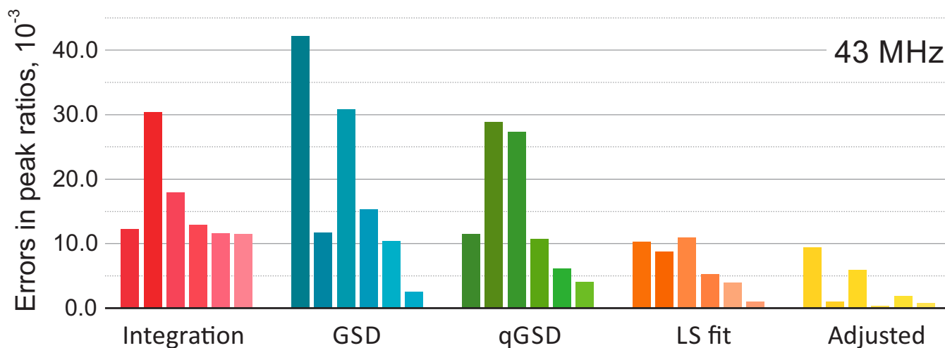
Figure 9. The results of quantitative analysis of thiamine spectra acquired on a high field (top) and medium field (bottom) spectrometers. The plots show absolute errors in ratios of peak intensities estimated with five different methods: the traditional peak integration, global spectral deconvolution (GSD) and its quantitative modification (qGSD), least-squares model fitting (LS), and the proposed adjustment algorithm applied to the LS fit. In each group, the bars correspond to the peaks of thiamine ordered from left to right according to their chemical shift. Note that the adjustment method improves the accuracy of model-based quantification for all peaks in both cases.
