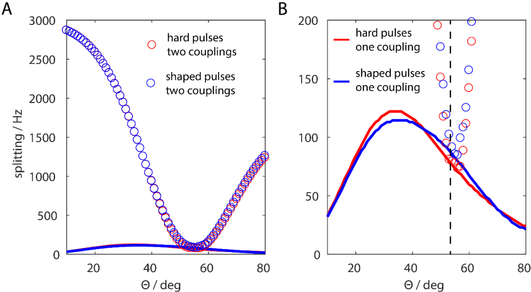
245 Figure 4: Calculated residual splitting of FSLG sequence in a homonuclear three-spin system as a dependence of the effective-field angle and implementations using rectangular pulses (red) and shaped pulses (blue). The splitting due to the residual coupling is shown without chemical-shift scaling due to the effective field axis. The second-order cross terms are minimized around the magic angle (circles) but the third-order terms resulting from a single dipolar coupling are never fully removed (solid line). A) Full scale of splitting as a function of the effective-field angle. B) Zoom on the residual splitting contributions up to 200 Hz. The MAS frequency was set to 6.25 kHz, the effective field to 125 kHz, the relative dipole orientation to 45^\circ , the dipolar couplings to 40 kHz for the single coupling and to 10 kHz for the second coupling, and powder averaging was applied. The black dashed line represents \theta = \theta_m .
