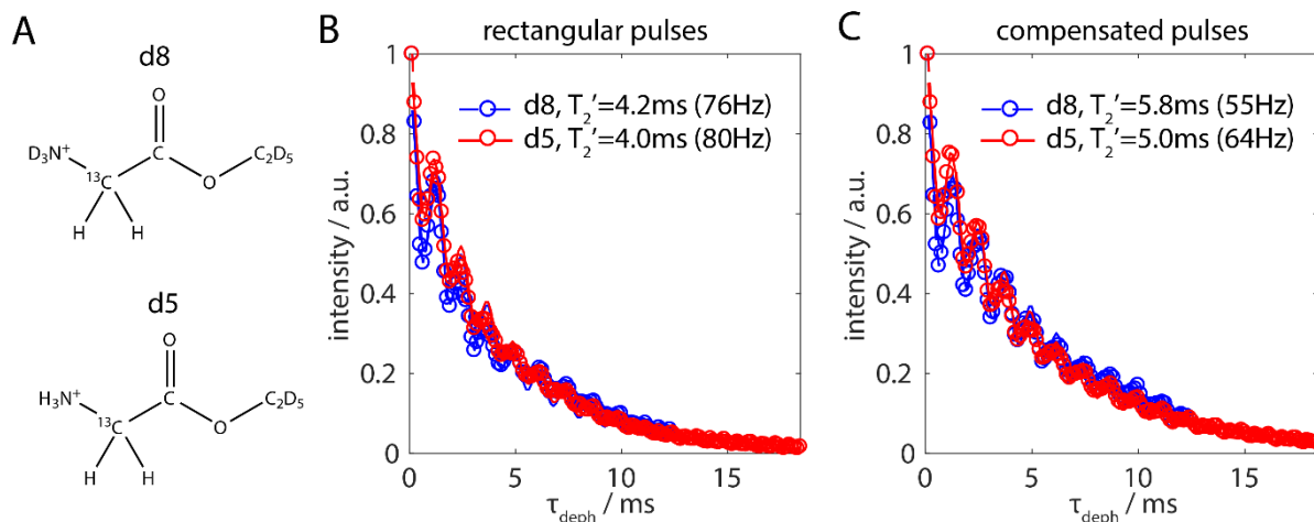
325 Figure 7: Quantification of the second- and third-order error terms in the FSLG pulse sequence. A) Model compounds of glycine ethylester with an isolated CH 2 -spin system (d8) and protonated representing a multi-spin system (d5). B) T_2' decay curves of the CH 2 -signal using FSLG decoupling on the protons during the echo time with rectangular pulses during the echo period and an effective-field angle equal to the magic angle. C) The identical curves to B) but using compensated pulses. The corresponding full width at half maximum is given in the figure legend. The MAS frequency was set to 14 kHz with an effective field of 125 kHz at an external magnetic field of 14.1 T.
