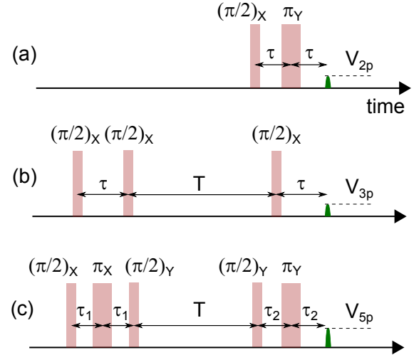
Figure 1. Sequences used for 2-pulse (a), 3-pulse (b), and 5-pulse (c) ESEEM measurements.
