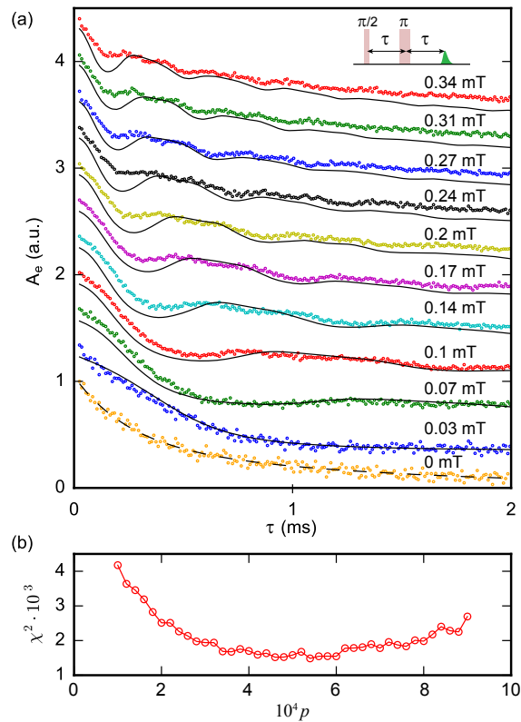
Figure 9. Two-pulse ESEEM of Bi:Si donors. (a) Echo integral A_e versus inter-pulse delay \tau for a 2-pulse echo sequence, for varying magnetic field B_0 . Dots are experimental data, lines are results of the model (see text), assuming a concentration in ^{29}\text{Si} of p = 4.4 \cdot 10^{-4} . The curves are vertically shifted, for clarity. (b) Fit residue \chi^2 for different ^{29}\text{Si} relative abundance p . The best fit is obtained for p = 4.4 \pm 1 \cdot 10^{-4} , in agreement with the specified value.
