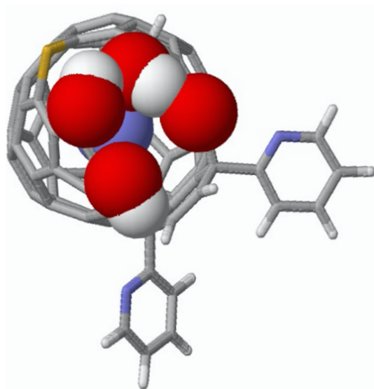
Figure A1. Top view on the DFT optimized structure of NO@C60-OH3 with N “up”. The modified C 60 cage is represented by sticks except van-der-Waals spheres for the oxygen and hydrogen atoms of the orifice and the caged NO (C (grey), H (white), N (blue), O (red), and S (yellow)).
