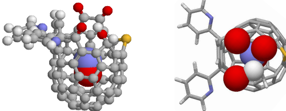
Figure 1. DFT optimized structure of NO@C60-OH1 with N “up”. Left: Ball-and-stick representation of the modified C 60 cage and van-der-Waals spheres of the caged NO with carbon (grey), hydrogen (white), nitrogen (blue), oxygen (red), and sulfur (yellow). Right: Top view on the orifice with stick representation of the cage except van-der-Waals spheres for the oxygen and hydrogen atoms of the orifice and the caged NO.
