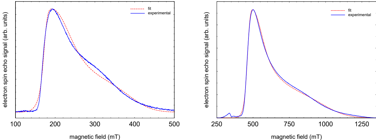
Figure 2. FSE spectra of NO@C60-OH1 ( T = 5 K) with best fits. Left: S band (3.5 GHz, 10 mM/CS 2 ). Right: X band (9.7 GHz, 2.5 mM/CS 2 ). For fitting a set of nitrogen hyperfine tensor parameters was used, determined by ENDOR (see below).
