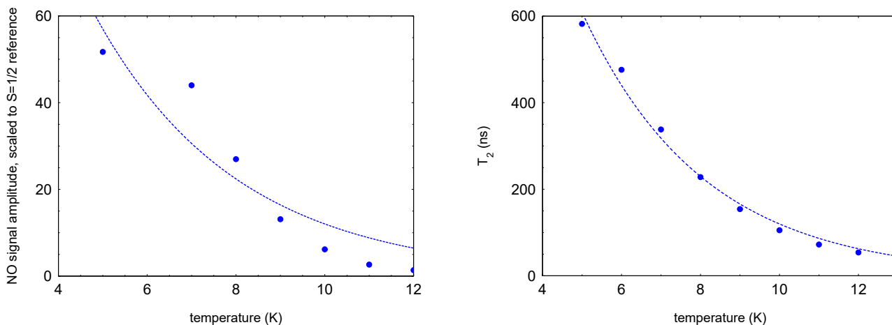
Figure 4. Echo-detected signal of NO@C60-OH3 (480 mT, 9.7 GHz, 2.5 mM/CS 2 , 200 ns pulse separation) as function of temperature. The signal intensity is scaled to the intensity of a field separated g \approx g_e signal from an unidentified S = 1/2 species following the Curie law. An exponential temperature dependence is assumed for the fit (dashed line) with a decay constant of 3 K. Right: Temperature dependence of the spin echo decay constant T_2 of NO@C60-OH3 (480 mT, 9.7 GHz, 2.5 mM/CS 2 ). The faster decay constant with larger weight is shown in cases where the time traces required a bi-exponential fit. Again an exponential temperature dependence is assumed for the dashed line, with a decay constant of 3.1 K.
