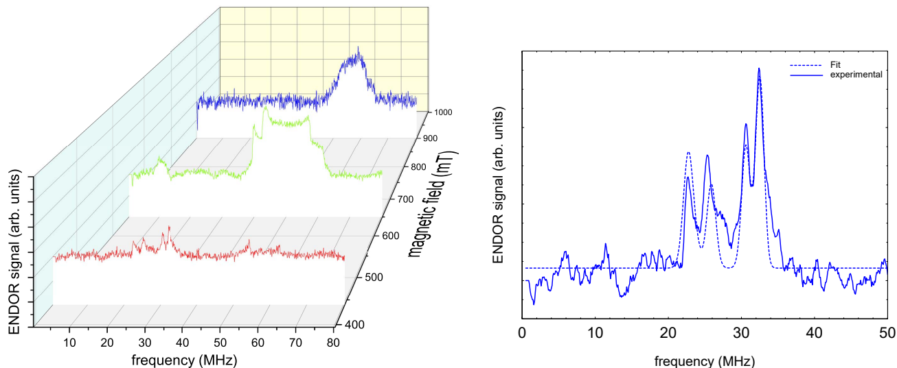
Figure 6. Left: Davies ENDOR spectra of NO@C60-OH1 ( T = 5 K, 10 mM/CS 2 ) measured as function of B_0 . Spectra are corrected with respect to different accumulation times for better comparison of spectral pattern. The Davies ENDOR pulse sequence (40-30000-20-200-40 ns, 25 \mu s rf pulse) was identical for all spectra. Right: ENDOR spectrum of NO@C60-OH1 measured at 440 mT (see left) together with simulation.
