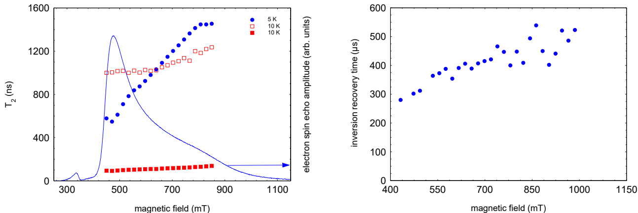
Figure 5. Left: Field and temperature dependence of 2-pulse echo decay of NO@C60-OH3. The 5 K data set could be satisfactorily fitted assuming a single exponential; the 10 K data required a bi-exponential fit. Both components were of similar magnitude, with the shorter T_2 larger in amplitude. Right: Field dependence of T_1 of NO@C60-OH3, measured using an inversion recovery pulse sequence at 3.6 K.
