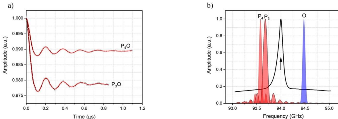
300 Figure 7: a) Background corrected DEER data (black curves) of Gd-ruler (2.1 nm) recorded with different offsets between pump and observer pulses together with fits (red curves) obtained by DeerAnalysis (2019) (Jeschke et al., 2006). b) Excitation profiles of the pump (P) and observer (O) pulses at different frequency offsets. The corresponding frequency offsets are P_3O = 800 MHz and P_4O = 900 MHz. The black arrow indicates the position of 94 GHz, the nominal centre frequency of our W- band EIK amplifier, which has a bandwidth of just less than 1 GHz.
