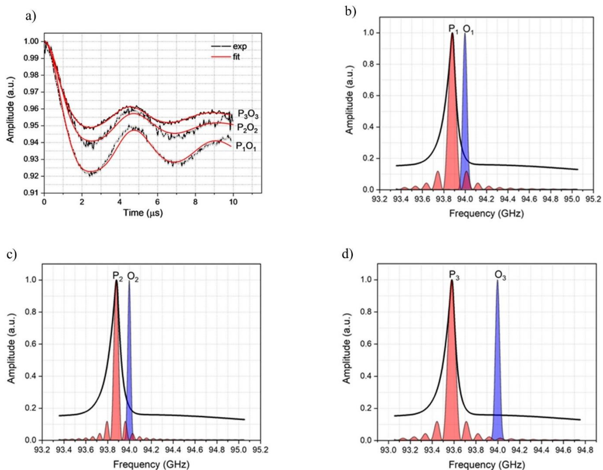
Figure 3: a) Background corrected DEER data (black curves) of Gd-ruler (6.0 nm) recorded with different PO offsets with the fits (red) obtained by DeerAnalysis (2019) (Jeschke et al., 2006). Excitation profiles of the pump (P) and observer (O) at different frequency offsets, b, c) P_1O_1 = P_2O_2 = 120 MHz with softer pulses for P_2O_2 and d) P_3O_3 = 420 MHz.
