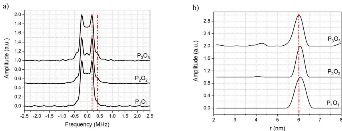
Figure 4: a) Pake pattern spectra obtained from fitting of the DEER data of the Gd-ruler (6.0 nm) sample measured with different offsets between pump and observer pulses and b) corresponding distance distributions derived from the DEER data. The PO offsets are P_1O_1 = P_2O_2 = 120 MHz and P_3O_3 = 420 MHz. The red vertical dashed lines show in a) the positions of the parallel and perpendicular singularities of the Pake pattern and in b) the expected distance. 260
