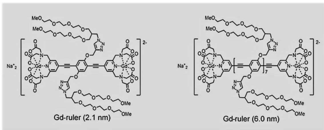
Figure 1: Chemical structures of Gd-ruler systems used in the current study.
