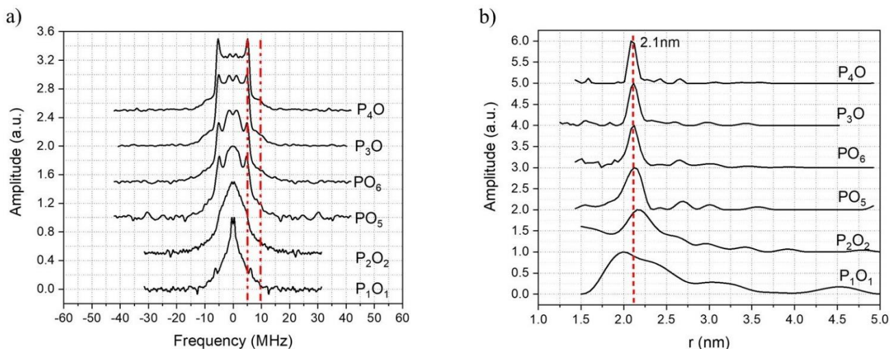
Figure 6: a) Pake pattern spectra obtained from the fitting of the DEER data of the Gd-ruler (2.1 nm) sample measured with different offsets between pump and observer pulses and b) associated distance distributions derived from the DEER data. The 290 corresponding frequency offsets are P 1 O 1 = 120 MHz, P 2 O 2 = 420 MHz, PO 5 = 840 MHz, PO 6 = 900 MHz, P 3 O = 800 MHz and P 4 O = 900 MHz. The red vertical dashed lines show in a) the positions of the parallel and perpendicular singularities of the Pake pattern and in b) the expected distance.
