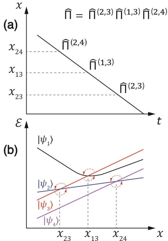
260 Figure 3. (a) Variation of the control parameter x with time. When the x value reaches the LACs region, mixing of the populations occurs, LC positions x_{kl} are indicated as well as the permutation operators. (b) Representation of the population mixing between the pairs of diabatic states at the corresponding LACs, indicated by arrows.
