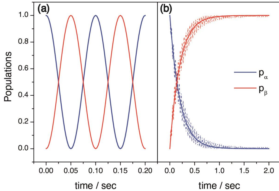
175 Figure 2. (a) Time dependence of the state populations in the case of coherent exchange with \omega_x/2\pi = 10 Hz, as obtained from eq. (7). (b) Populations after a passage through zero field, \omega_z = 0 , as functions of the switching time \tau_{sw} . Here the solid lines present the result of eq. (8) and the dashed lines show the numerical simulation result. Here \omega_x/2\pi = 10 Hz, \omega_z^{max}/2\pi = 100 Hz. Initially the system is in the |\alpha\rangle state; the blue and red lines shown the populations of the |\alpha\rangle and |\beta\rangle states, respectively.
