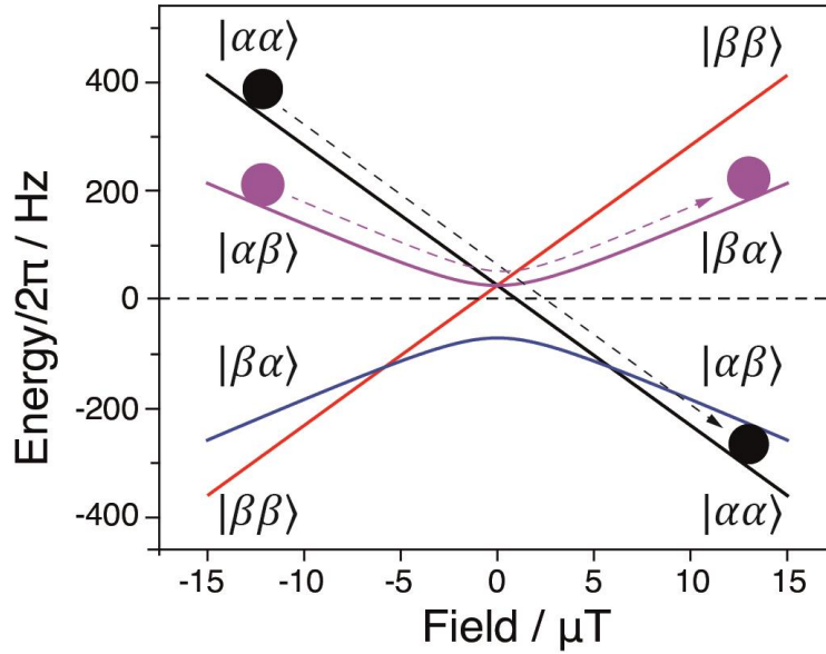
320 Figure 4. Correlation diagram for an adiabatic inversion. Simulation parameters: J_{IS} = 100 Hz, I and S spins are ^1\text{H} and ^{13}\text{C} nuclei with the gyromagnetic ratios \gamma_H = 2.68 \cdot 10^8 rad·s ^{-1} ·T ^{-1} and \gamma_C = 6.73 \cdot 10^7 rad·s ^{-1} ·T ^{-1} .
