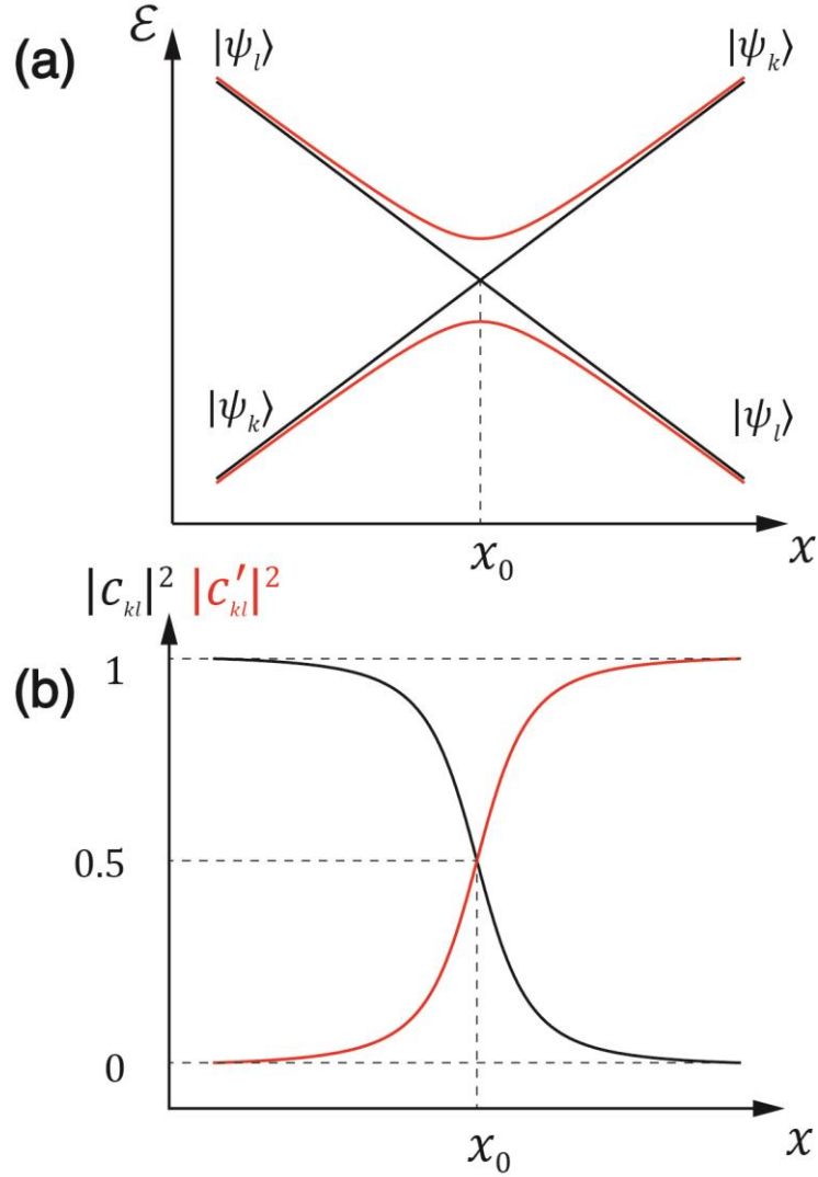
110 Figure 1. (a) Representation of an LC and LAC. The black lines represent the energies of the diabatic states, which have a LC. The red lines show the adiabatic energy levels. (b) The mixing coefficients introduced in eq. (3) in the LAC region.
