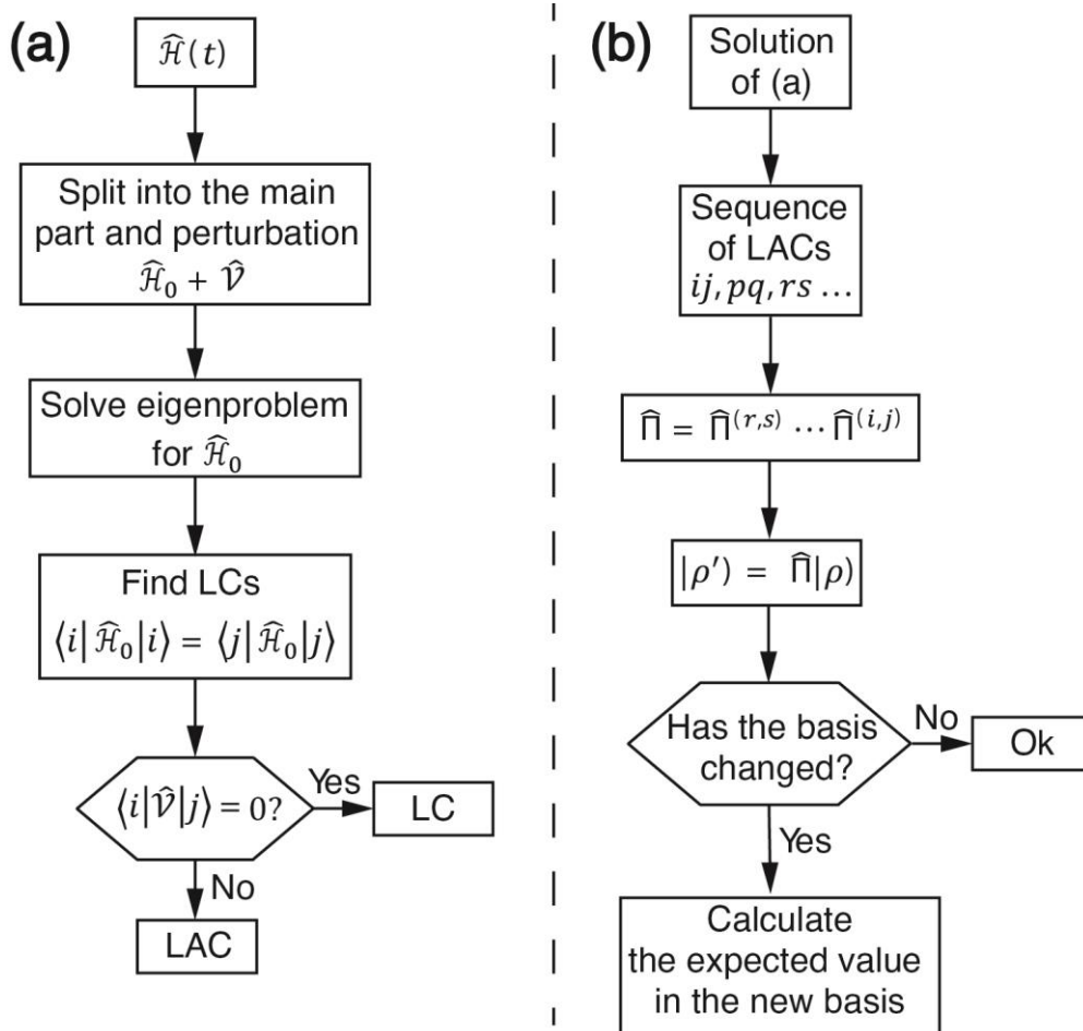
630 Figure 9. Flow-chart diagram indicating (a) the way to find all LACs and (b) to calculate the spin dynamics due to LACs.
