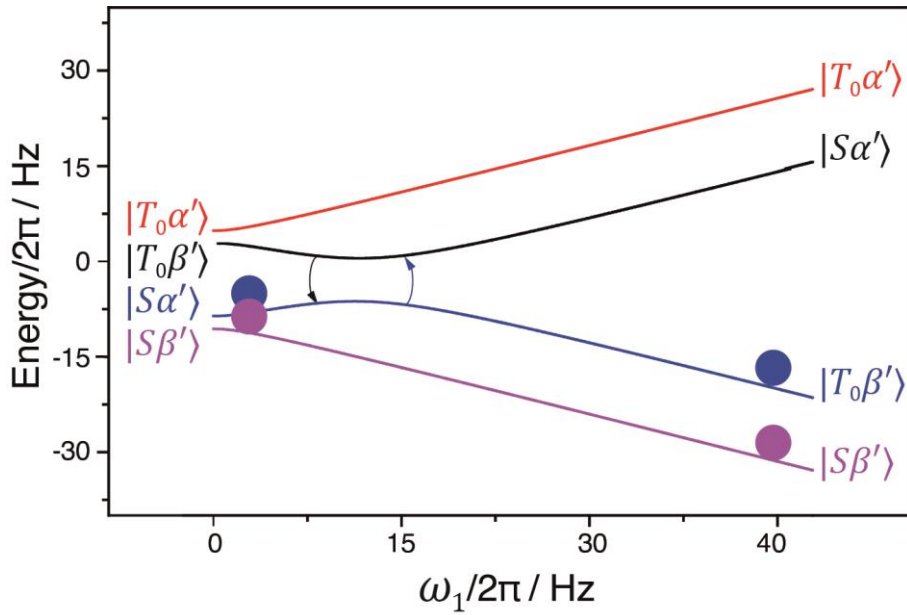
Figure 8. Population swapping upon increase of the amplitude of the RF-field applied to the S spin. Simulation parameters: I and S nuclei are ^1\text{H} and ^{13}\text{C} respectively, J_{II} = 11.5 Hz, J_{IS} = 13.7 Hz, \delta\omega = 2 Hz. See text for further detail.
