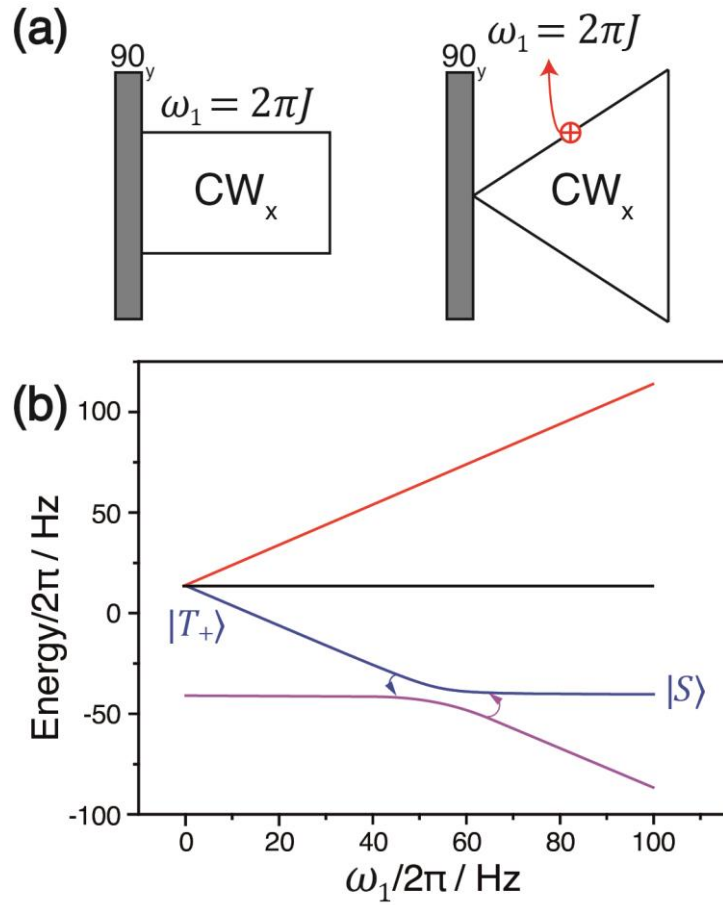
490 Figure 7. (a) The experimental protocol of SLIC (left) and adiabatic SLIC with linearly ramped RF-field amplitude (right). (b) Correlation diagram describing T_+ \rightarrow S conversion at the LAC.
