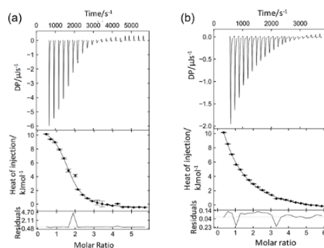
Figure S1. Representative isothermal titration calorimetry experiments of ubiquitin E18Sep titrated with LnCl 3 . (a) Cell = 150 μM ubiquitin E18Sep; syringe = 2.7 mM TbCl 3 . (b) Cell = 150 μM ubiquitin E18Sep; syringe = 2.7 mM TmCl 3 . The top panel shows the baseline-corrected power traces. The middle panel displays the heat data and best fit. The bottom panel shows the residual of the fit. Error bars calculated by the program NITPIC (Keller et al., 2015) indicate the standard error in the integration of the peaks. DP denotes the power differential between the reference and sample cells to maintain a zero temperature difference between the cells.
