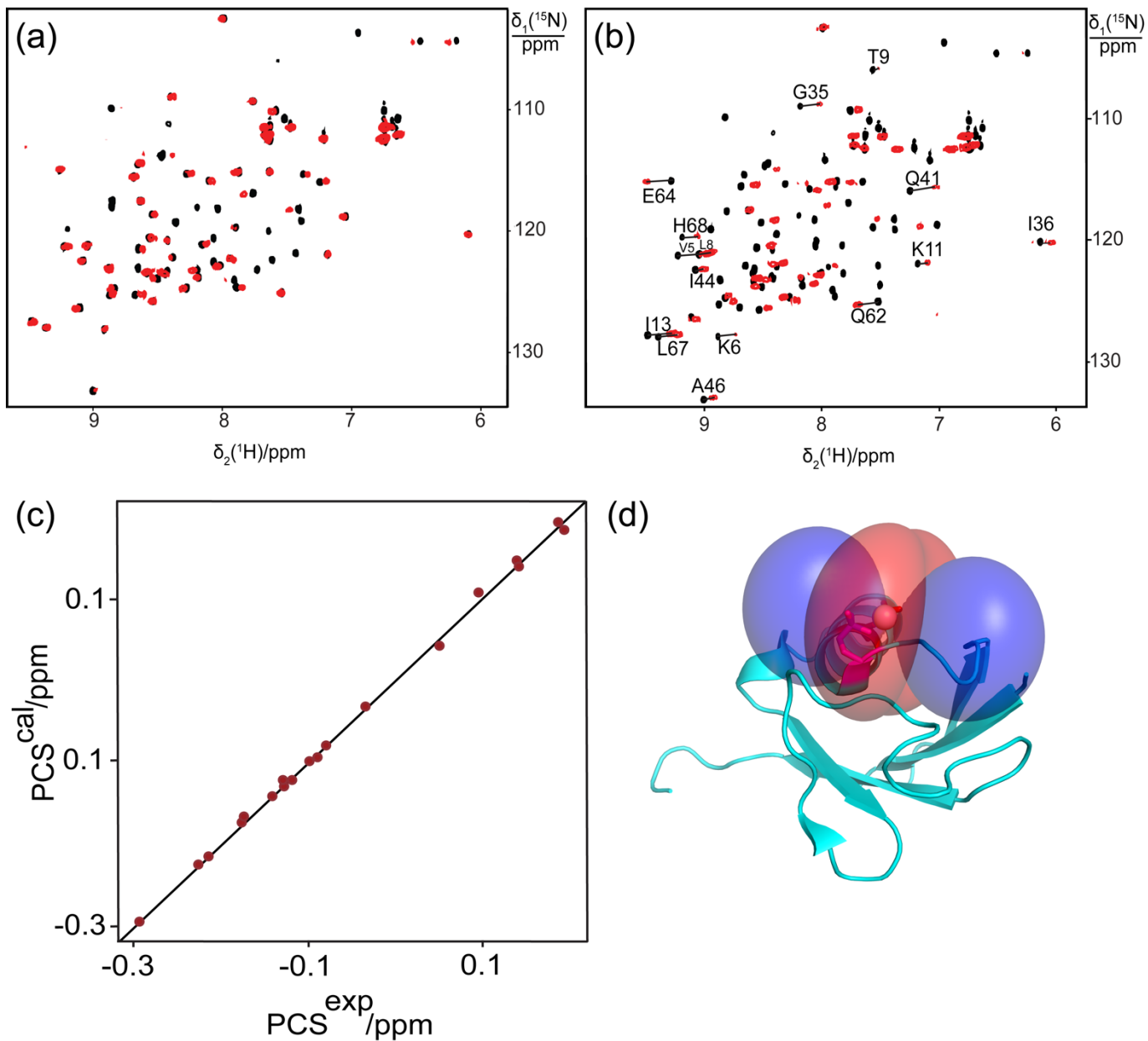
320 Figure 7. Breaking a salt bridge in ubiquitin T22Sep/N25D generates a specific lanthanide binding site. (a) Superimposition of [^{15}\text{N}, ^1\text{H}] -HSQC spectra of 0.3 mM solutions of ubiquitin T22Sep/N25D recorded in the presence of \text{Tb}^{3+} (red) or \text{Y}^{3+} (black).
