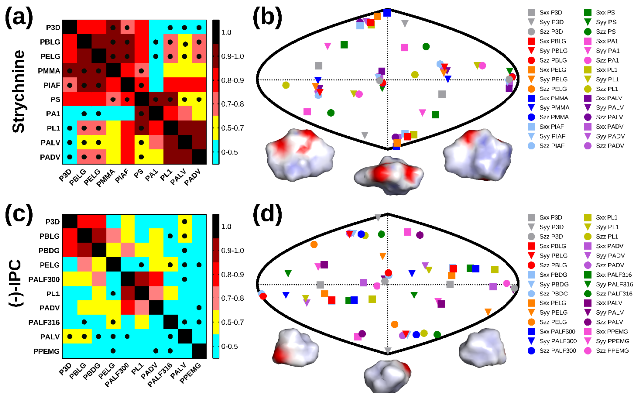
225 Figure 3: RDCs and alignment comparison of different alignment media and P3D for strychnine and (-)-IPC. (a, c) Matrices of Pearson's correlation R between P3D-calculated RDCs and the experimental RDCs in different alignment media for strychnine (a) and (-)-IPC (c). Dots mark negative correlations. (b, d) Comparison of the orientation of the P3D-predicted alignment tensor (grey) with alignment tensors derived by SVD from experimental RDCs of the different alignment media for strychnine (b) and (-)-IPC (d). The orientation of the three axes corresponding to the eigenvalues Szz (circle), Syy (triangle) and Sxx (square) of the diagonalized alignment tensor are projected onto a two-dimensional world map. Different orientations of the charged surface of strychnine (b) and (-)-IPC (d) are shown below.
