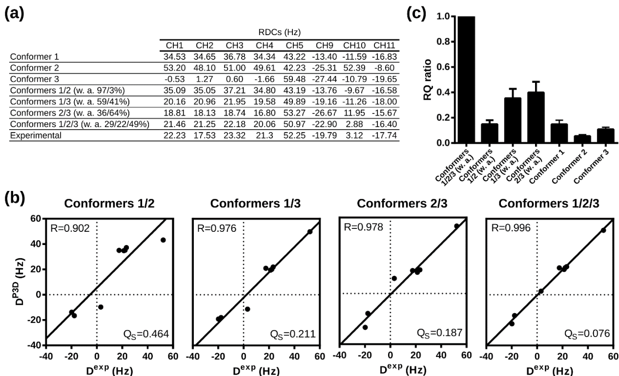
355 Figure 6: P3D-based refinement of the conformational ensemble of sucrose. (a) List of P3D-calculated RDCs for the 3 conformers together with the average weighted RDCs from the RQ maximization for 2- and 3-conformer ensembles and the experimental RDCs. (b) Correlation between the experimental RDCs ( D^{\text{exp}} ) and the P3D-calculated RDCs for the weighted average of the RQ maximization for 2- and 3-conformer ensembles. (c) RQ ratios of the three different conformers in reference to their weighted average as 2- and 3-conformer ensembles. Error bars were calculated as the propagation of R and Q_S errors and these errors are 360 calculated from the std of 100 repetitions including noise in the RDCs.
