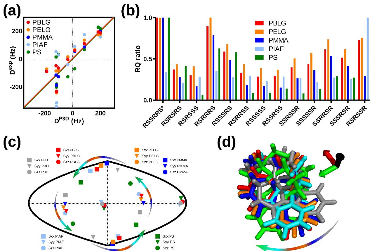
245 Figure 4: P3D and the alignment media with most similar alignment properties for strychnine. (a) Correlation between P3D-simulated RDCs ( D^{P3D} ) and experimental RDCs ( D^{exp} ) with different alignment media for strychnine. Experimental values are normalized by the slope of the linear fitting. (b) Diastereomer discrimination power of different alignment media for strychnine based on the P3D simulation and using the RQ ratio for judging the quality of correlation. (c) Comparison of the orientation of the P3D-predicted alignment tensor (grey) of strychnine with alignment tensors derived by SVD from the experimental RDCs using PALES (Zweckstetter, 2008) observed in different alignment media. The orientation of the three axes corresponding to the eigenvalues Szz (circle), Syy (triangle) and Sxx (square) of the diagonalized alignment tensor are projected onto a two-dimensional
