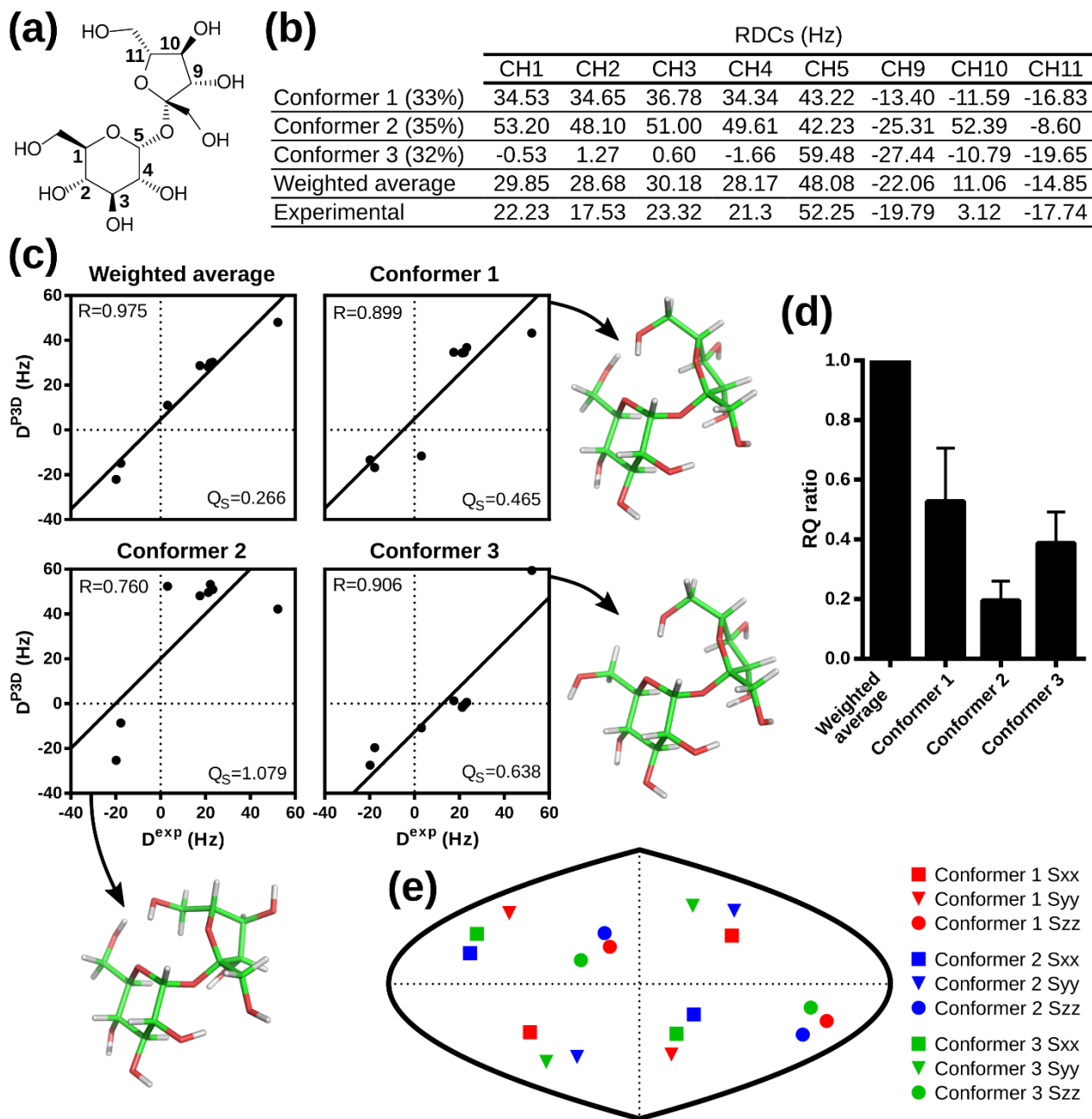
Figure 5: Validation of the conformational ensemble of sucrose using P3D. (a) Sucrose structure with the CH carbons labeled. (b) List of P3D-simulated RDCs for the 3 conformers together with the average weighted RDCs (from Ndukwe et al. populations) and the experimental RDCs. (c) Correlations between the experimental RDCs ( D^{\text{exp}} ) and the P3D-simulated RDCs for the 3 conformers and the weighted average. (d) RQ ratios of the 3 different conformers in reference to the weighted average. Error bars are calculated as the propagation of R and Q_S errors and these errors are calculated from the std of 100 repetitions including noise in the RDCs.
