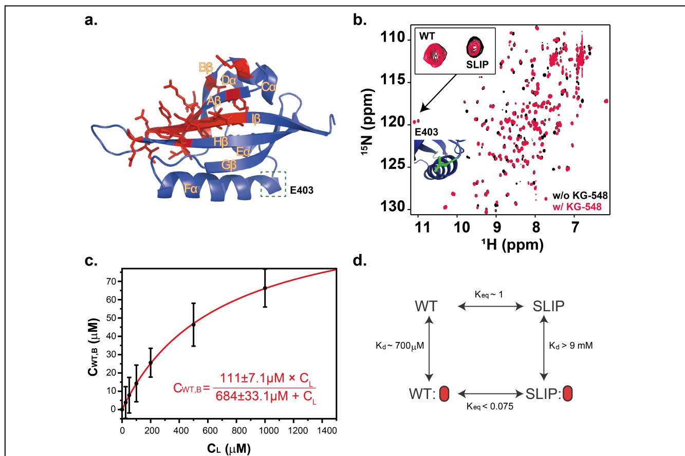
Figure 5 – Characterization of KG-548 binding to ARNT PAS-B Y456T and impact on WT:SLIP conformation.
