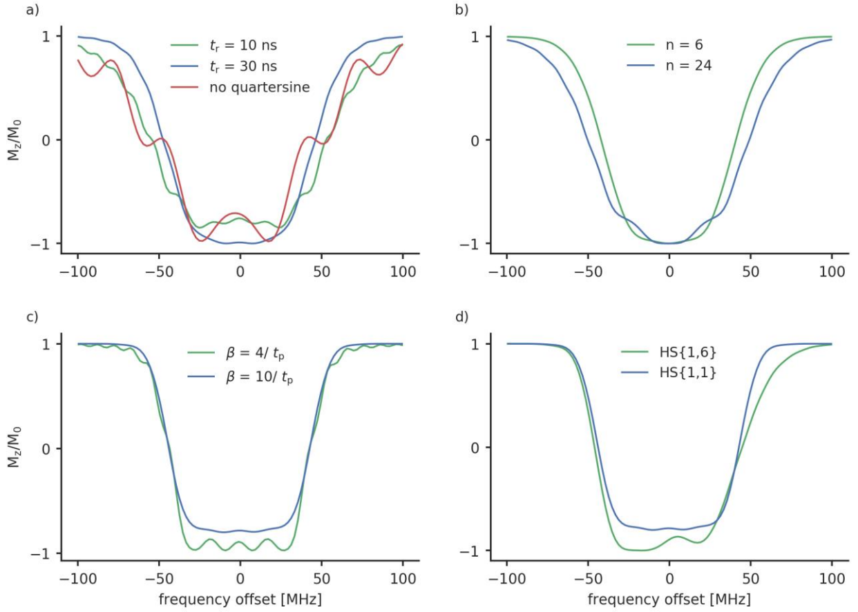
Figure 3: Calculated inversion profiles of broadband pulses normalised to \nu_1 = 30 MHz, which corresponds to the maximum of the measured resonator profile. a) Chirp pulses with a frequency width of 120 MHz, a length of 100 ns and a rising time of 10 ns (green), a rising time of 30 ns (blue), a length of 36 ns and no quarter sine smoothing (red). b) WURST pulses with a frequency width of 120 MHz, a pulse length of 100 ns and a value for n of 6 (green) and 24 (blue). c) HS{1,1} pulses with a frequency width of 90 MHz and a truncation parameter of 4 (green) and 10 (blue). d) An HS{1,6} (green) and HS{1,1} (blue) pulse with a width of 90 MHz and a pulse length of 100 ns. The truncation parameter was 10 in both cases.
