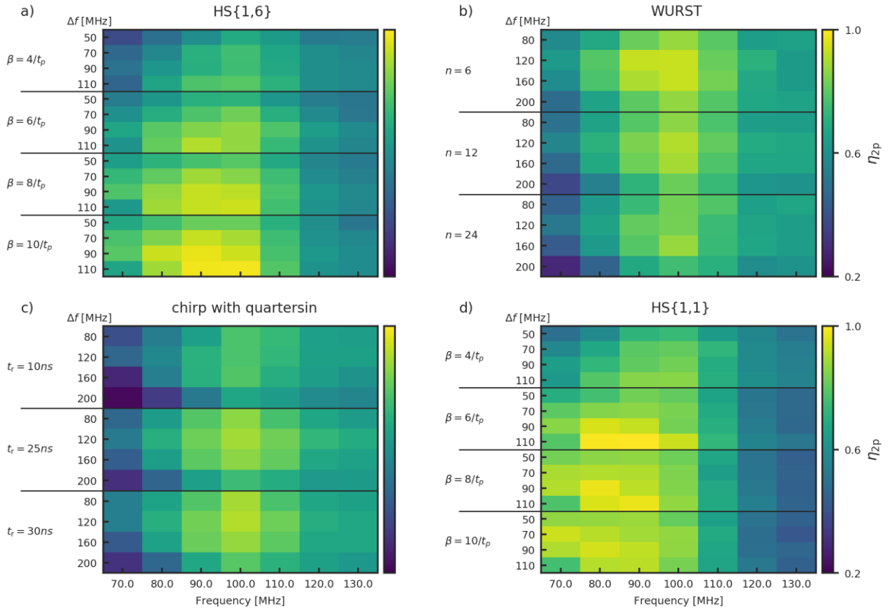
Figure 5: Heat maps with the \eta_{2p} - values for 4p-DEER measurements with an observer pulse length of 56 ns, Gaussian pulses and an integration window of 56 ns. The observer frequency is at 33.93 GHz. The pump pulse length is 100 ns. Each heat map shows a different pump pulse type: (a) HS{1,6}, (b)WURST , (c) chirp with quarter sine, and (d) HS{1,1}.
