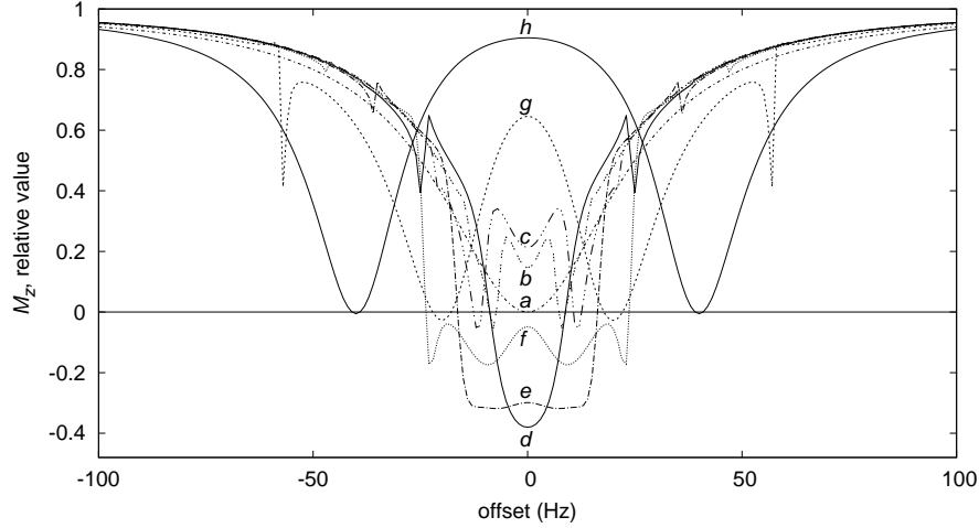
Figure 2. Saturation profiles for presaturation at two sites, at \pm\Omega^{\text{sat}}/2\pi for \Omega^{\text{sat}}/2\pi = 0, 2, 4, 6, 8, 10, 20, 40 Hz, corresponding to traces a to h. The relaxation times T_1 and T_2 are both equal to 0.5 s. The relaxation delay lasts 5 s during which 10 presaturation modules of 0.5 s each are applied. Each module is made of 50000 slices, for which \Omega_{1x} and \Omega_{1y} values are calculated with \Omega_1/2\pi = 50 Hz.
