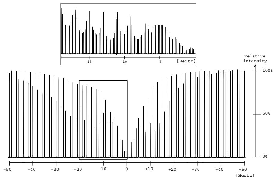
Figure 7. Presaturation profile in the region of two oxygen-bearing carbons for the 1,2-propanediol. A focus is made between 0 and -20 Hz to make the wavy part of the profile more visible.
