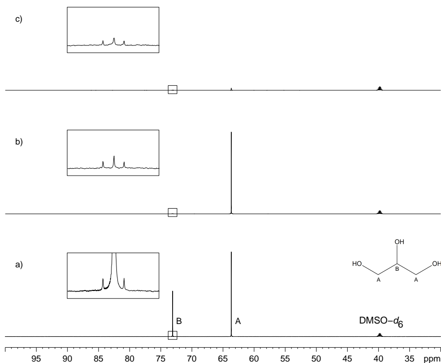
Figure 5. Presaturation of glycerol in DMSO- d_6 . a) ^{13}\text{C} NMR spectrum of glycerol. Signals from sites A and B are located at \delta_A 63.7 and \delta_B 73.1. b) Effect of single presaturation at site B. c) Effect simultaneous presaturation at sites A and B. The presaturation module last T = 1 s and are applied with a maximal intensity \Omega_1/2\pi of 11.7 Hz All acquisitions required the recording of 8 scans preceded by 4 dummy scans.
