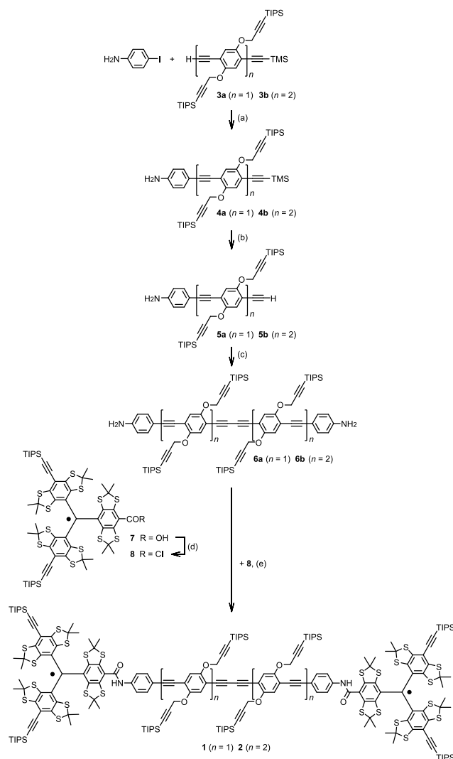
Figure 2. Synthesis of the bis-trityl rulers 1 and 2 . For n = 1 : (a) \text{PdCl}_2(\text{PPh}_3)_2 , \text{CuI} , piperidine, THF, rt, 25 h, 84%; (Ritsch et al., 2019) (b) \text{K}_2\text{CO}_3 , MeOH, \text{CH}_2\text{Cl}_2 , rt, 14.5 h, 96%; (c) \text{PdCl}_2(\text{PPh}_3)_2 , \text{CuI} , piperidine, THF, air, rt, 16 h, 36%; (d) \text{SOCl}_2 , \text{CHCl}_3 , 50 °C, 90 min, not isolated; (e) ^i\text{Pr}_2\text{NEt} , \text{CHCl}_3 , rt, 17 h, 40%. For n = 2 : (a) \text{PdCl}_2(\text{PPh}_3)_2 , \text{CuI} , piperidine, THF, rt, 46 h, 86%; (b) \text{K}_2\text{CO}_3 , MeOH, \text{CH}_2\text{Cl}_2 , rt, 14.5 h, 96%; (c) \text{PdCl}_2(\text{PPh}_3)_2 , \text{CuI} , piperidine, THF, air, rt, 15.5 h, 65%; (d) \text{SOCl}_2 , \text{CHCl}_3 , 50 °C, 90 min, not isolated; (e) ^i\text{Pr}_2\text{NEt} , \text{CHCl}_3 , rt, 19 h, 64%. For further details see the SI part B. THF = tetrahydrofuran, TIPS = triisopropylsilyl, TMS = trimethylsilyl, rt = room temperature.
