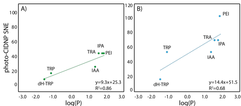
250 Figure 4: Correlation between the molecule hydrophobicity and the photo-CIDNP performances for the tryptophan derivatives. A) In the case where CW-photo-CIDNP is monitored by AT12. B) In the case where CW-photo-CIDNP is monitored by fluorescein. Log(P) is the logarithm of the partition coefficient, P, between octanol and water and were calculated with DataWarrior®. A statistical analysis of the trendlines using Pearson's R coefficient and the Student t-test for the hypothesis shows that for AT12 (A) a t of 4.87 and a p-value of 0.008 and for fluorescein (B) a t of 2.6 and a p-value of 0.060 is obtained. Hence, in both cases, the hypothesis H0 (absence of correlation) is rejected, and the alternative hypothesis (correlation is non-null) is retained.
