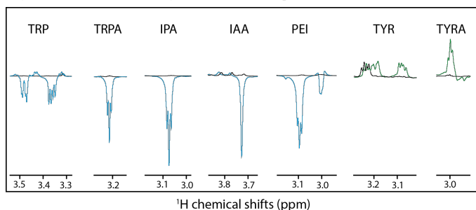
230 Figure 3: H_{\beta} anomalous signals for the different molecules. Dark lines are the reference spectra and blue lines are the irradiated spectra in the presence of fluorescein, and the green lines are the irradiated spectra in the presence of AT12. Scales between the different molecules are not respected for clarity purposes.
