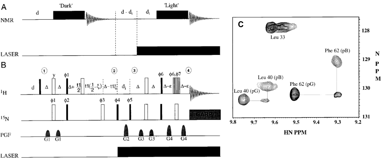
380 Figure 6: General NMR scheme for the study of pB (A), ^{15}\text{N} -SCOTCH subsequence for HSQC assignment (B). (C) Superimposed regions of the HSQC spectra of pG, pB, and the ^{15}\text{N} -SCOTCH exchange experiment connecting the HSQC cross peaks. Reproduced with permission from Elsevier (Rubinstenn et al., 1999)
