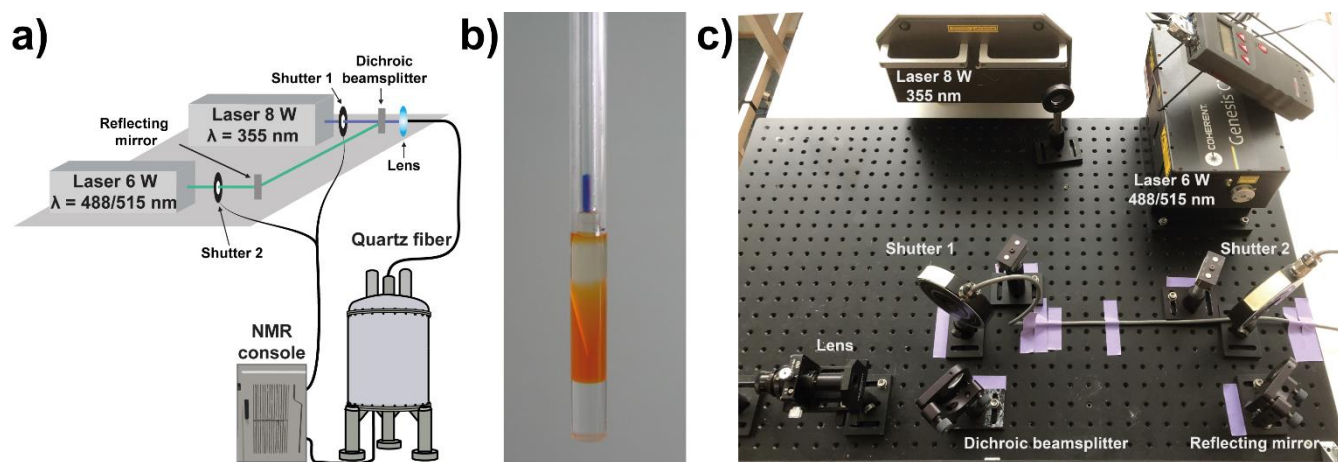
180 Figure 3: Setup to trigger real-time NMR experiments with in situ light induction. a) Schematic representation of a two-source setup for high-power laser irradiation connected to a NMR tube via a quartz fiber. The shutters can be directly triggered via the NMR console/pulse programme. b) Shigemi tube with cone shaped quartz tip for homogeneous sample illumination (Kühn and Schwalbe, 2000). The glass fiber can be inserted into the plunger. c) Two-wavelength laser setup installed at BMRZ, Frankfurt.
