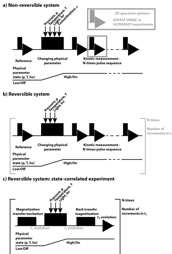
240 Figure 5: General pulse schemes used for RT-NMR measurements. In all cases first reference spectrum is measured, followed by a rapid trigger using corresponding physical parameter change. In a) general scheme is shown for non-reversible systems and in b) reversible systems are shown. In c) SC-spectrum experiments are shown, suitable for reversible systems to study rapid changes (< 1 sec). T_1 evolution time can be introduced either before or after the trigger part.
