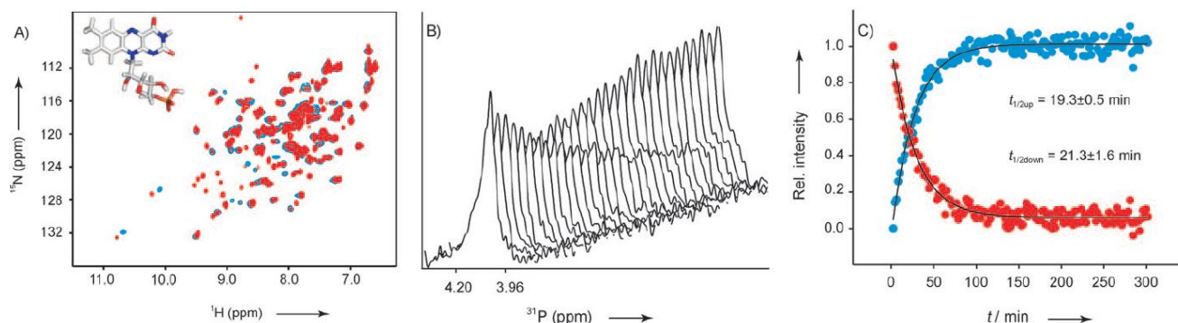
Figure 7: a) ^1\text{H} , ^{15}\text{N} HSQC of YcgF (reconstituted with FMN) in the dark (blue) and light (red) state. b) ^{31}\text{P} stack plot representations of the chromophore after light illumination. c) Normalized and fitted signal intensities of ^{31}\text{P} kinetics traces for t_{1/2} calculations. Reproduced with permission from Wiley (Schroeder et al., 2008)
