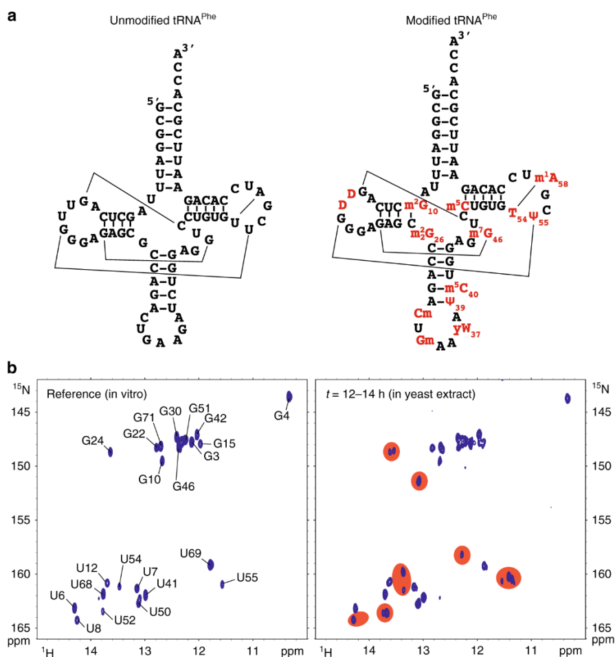
Figure 15: A RNA secondary structure of unmodified and modified tRNA Phe a sequence and cloverleaf representation of unmodified yeast tRNA Phe (left) and modified tRNA Phe (right). b) 1 H- 15 N HSQC spectra in vitro (left) and upon 12 h after addition to yeast extract. Assignments are indicated in the in vitro spectrum while red patches highlight areas with significant changes. Reprinted from (Barraud et al., 2019)
