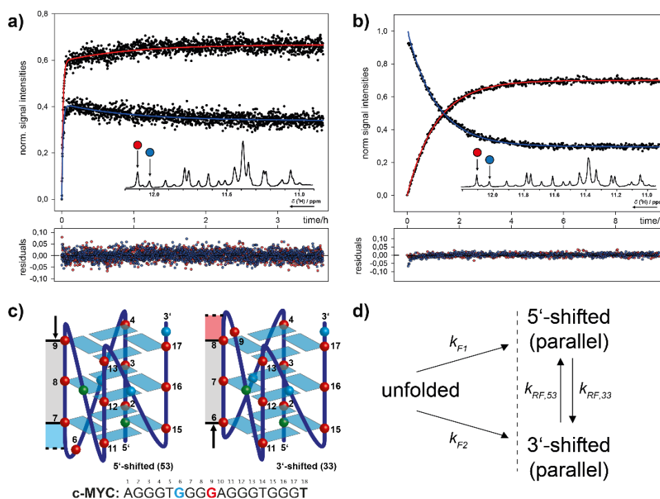
640 Figure 13: Combinatorial study of folding and refolding of a 18-mer DNA G-quadruplex (G4) forming oligonucleotide sequence from the human cMYC proto-oncogene promoter by (Grün et al., 2020). (a) Parallel folding of two coexistent G4 conformations, induced by in situ rapid-mixing with \text{K}^+ -ions that are required for G4 formation. (b) Refolding of photocaged, isolated G4 645 conformations back into conformational equilibrium. (c) Schematic representation of the two coexisting G4 conformations distinguished by a register shifted G-rich strand. (d) Kinetic model for parallel folding into two coexisting conformations and subsequent refolding dynamics in conformational equilibrium. Reprinted (adapted) with permission from J. Am. Chem. Soc. 2020, 142, 1, 264–273. Copyright 2020 American Chemical Society.
