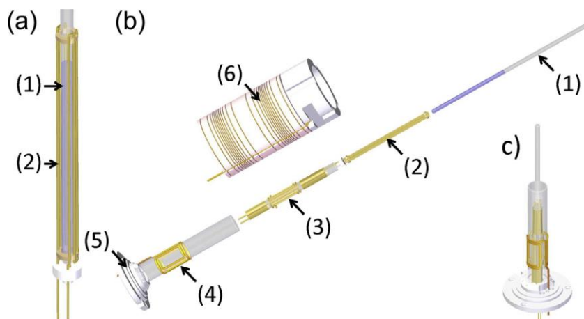
195 Figure 4: Schematic view of the coil assemblies in the T-jump probehead developed by (Rinnenthal et al., 2015). (a) Cage coil/wire capacitor for rf-heating with sample tube (2.5 mm), (b) exploded view of the overall assembly with (1) sample tube, (2) 2.5 mm cage coil, (3) 5 mm double tuned ( ^1\text{H} and ^2\text{H} ) rf NMR saddle coil, (4) 10 mm ( ^{15}\text{N} ) rf NMR saddle coil, (5) coil insert base and connection to main probe body, (6) z gradient coil. (c) Full assembly of coils in the T-jump probe (z gradient system not shown). Reproduced with permission from (Rinnenthal et al., 2015).
