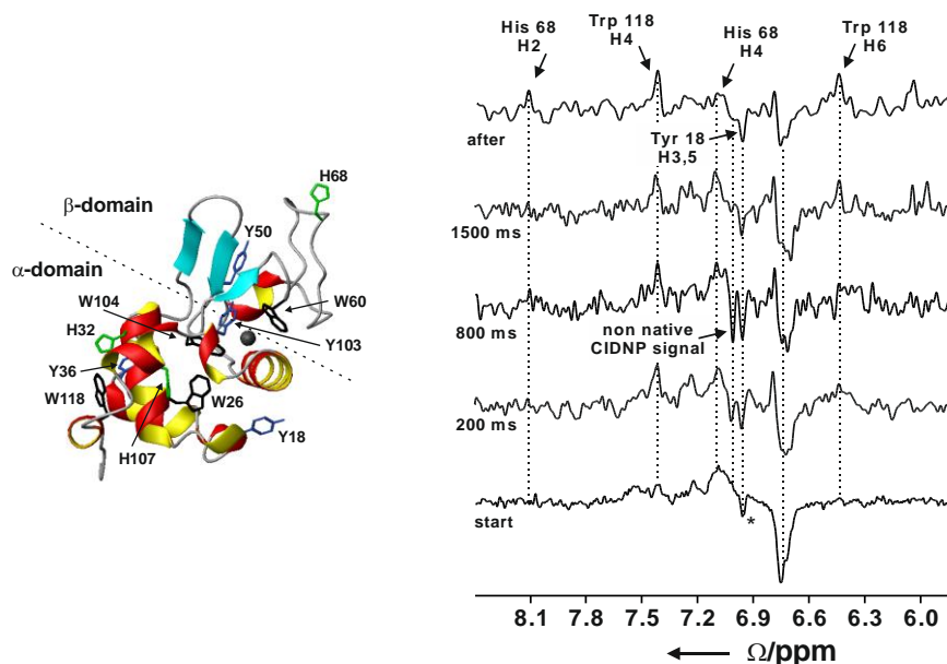
500 Figure 10: Time-resolved photo-CIDNP NMR of the refolding of bovine \alpha -lactalbumin at 4M urea upon the addition of \text{Ca}^{2+} using laser irradiation. Left: ribbon representation of the native structure of the protein (1HFZ.pdb) (Pike et al., 1996); * is the native signal of Tyr18 which is already present at the start of the experiment. Reproduced with permission from Wiley (Wirmer et al., 2001)
