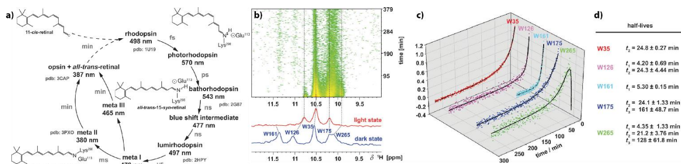
430 Figure 8: Analyses of the long lived meta III and meta II states of rhodopsin after illumination. a) The photocycle of bovine rhodopsin with the first detectable intermediate of photorhodopsin and subsequent intermediates as a product of thermal relaxation. b) Time series of ^1\text{H} -NMR spectra from the indole region of a selective \alpha,\epsilon - ^{15}\text{N} -tryptophan-labeled rhodopsin and corresponding dark state (blue) and light state (red). c) Time traces of the indole signal intensities and the corresponding half-lives 435 extracted from exponential fits to the time dependant signal intensities. The figure was adapted with permission from Wiley (Stehle et al., 2014).
