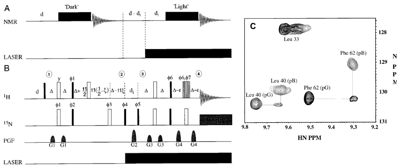
375 Figure 6: General NMR scheme for the study of pB (A), 15 N-SCOTCH subsequence for HSQC assignment (B). (C) Superimposed regions of the HSQC spectra of pG, pB, and the 15 N-SCOTCH exchange experiment connecting the HSQC cross peaks. Reproduced with permission from Wiley (Rubinstenn et al., 1999)
