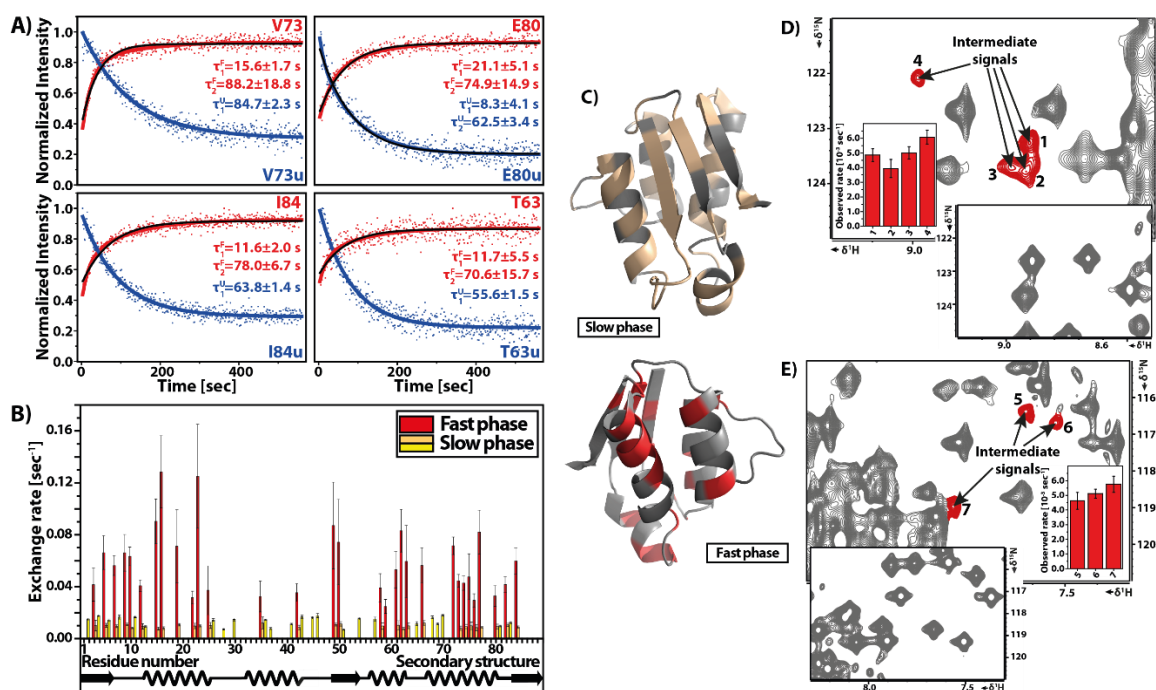
655 Figure 14: T-jump experiment on the cold denatured C40A/C82A barstar mutant. A) Representative time-dependent signal intensities with double exponential kinetic fit. B) Residue specific results of refolding kinetics. C) Three-dimensional structure of barstar (PDB: 1AB7) highlighting the affected residues with slow (pale yellow) and fast (red) phase of observed kinetics. D-E) Different part of the same ^1\text{H} - ^{15}\text{N} HSQC spectrum detected in slow T-jump experiment using gas-heating system with high sensitivity cryoprobe detected stable intermediate signals. Reproduced with permission from (Pintér and Schwalbe, 2020).
