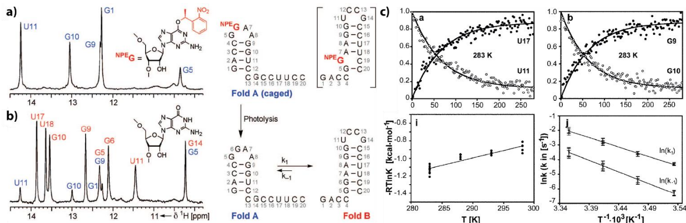
605 Figure 12 a) and b) ^1\text{H} NMR spectra of imino protons with color coding according to the secondary structure shown to the right. a) Spectrum of the conformationally locked Fold A (caged by introduction of O 6 -(S)-NPE modified guanosine at position 6). c) Top: representative normalized signal intensities as a function of time after release of native state by a single laser pulse. Down: Arrhenius analyses of k_1 and k_{-1} . Reproduced with permission from Wiley (Wenter et al., 2005)
