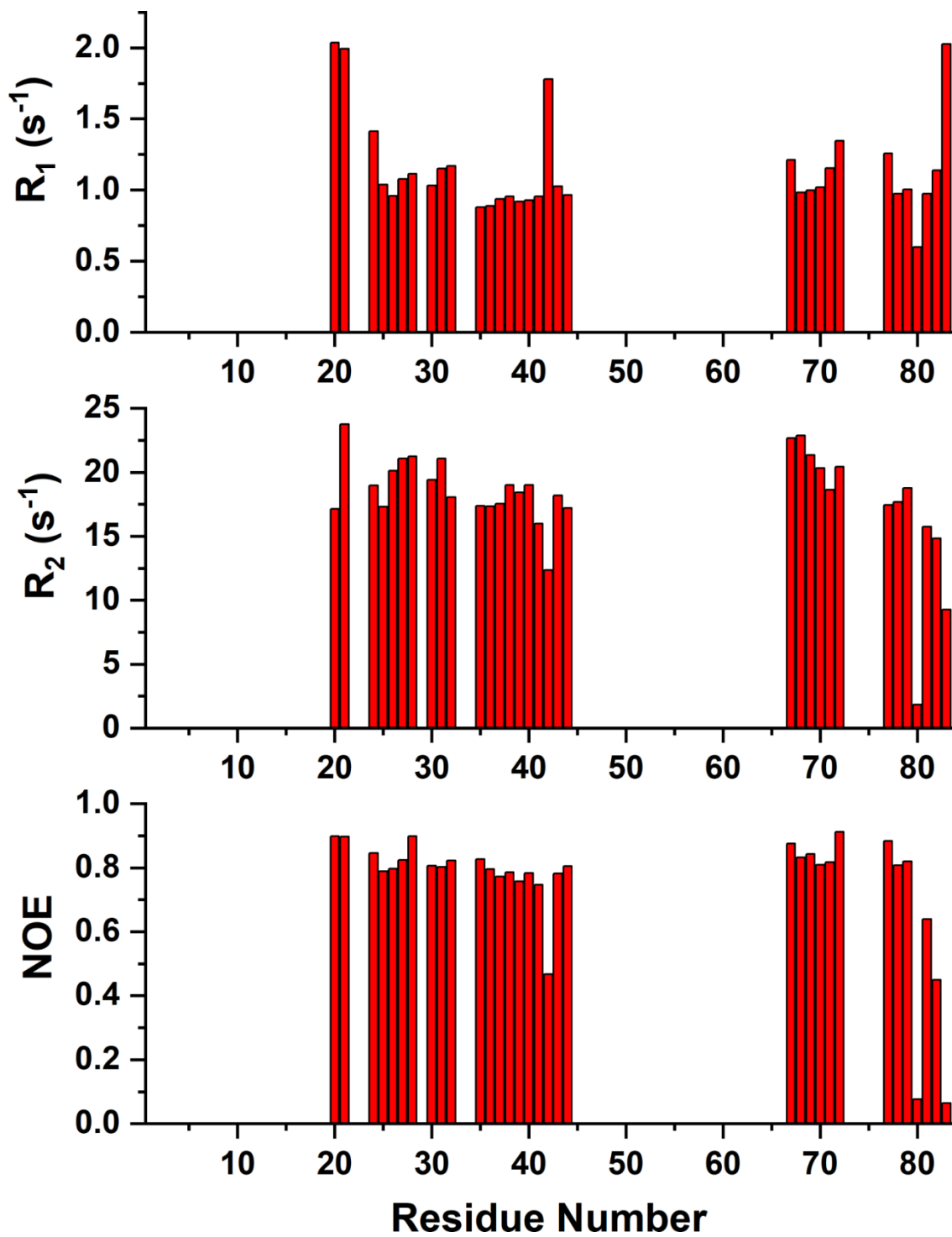
555 Figure A4: 15 N R_1 , R_2 , and 15 N{ 1 H} NOE values versus residue number of reduced mitoNEET obtained at 500 MHz and 298 K.
