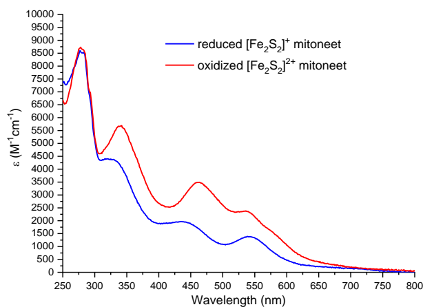
Figure A1: UV-visible spectra of reduced [Fe_2S_2]^+ - (blue line) and oxidized [Fe_2S_2]^{2+} - mitoNEET (red line). \epsilon values are based on monomeric protein concentration (determined with Bradford assay).
