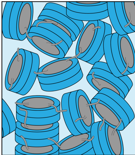
Figure 5. Schematic illustration of the packing in the nucleosome sediment obtained by ultracentrifugation. The packing density is the schematic corresponds to our experimental estimate (~61%), while the heterogenous orientation of nucleosomes in the sediment reflects the lack of strong long-order in the sample. Nucleosome-nucleosome interactions are predominantly formed by histone tail-DNA interactions.
