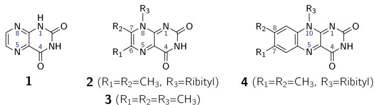
Scheme 1. Lumazine ( 1 ), 6,7-dimethyl-8-ribityllumazine ( 2 ), 6,7,8-trimethylumazine ( 3 ) and riboflavin ( 4 )
