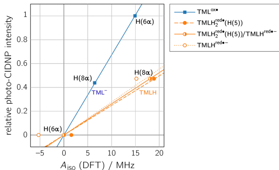
240 Figure 5: Correlations of relative photo-CIDNP intensities to predicted A_{\text{iso}} values from DFT. \text{TML}^{\text{ox}\bullet} : slope = 0.0672 \text{MHz}^{-1} , R^2 = 0.9996 ; \text{TMLH}^{\text{red}\bullet-} : slope = 0.0277 \text{MHz}^{-1} , R^2 = 0.7827 ; \text{TMLH}_2^{\text{red}\bullet}(\text{H}(5)) : slope = 0.0248 \text{MHz}^{-1} , R^2 = 0.9863 ; linear combination of \text{TMLH}_2^{\text{red}\bullet}(\text{H}(5)) and \text{TMLH}^{\text{red}\bullet-} with a ratio of 0.772:0.228: slope = 0.0262 \text{MHz}^{-1} , R^2 = 1 . CIDNP intensities were multiplied by the respective \text{sgn}(\Delta g) .
