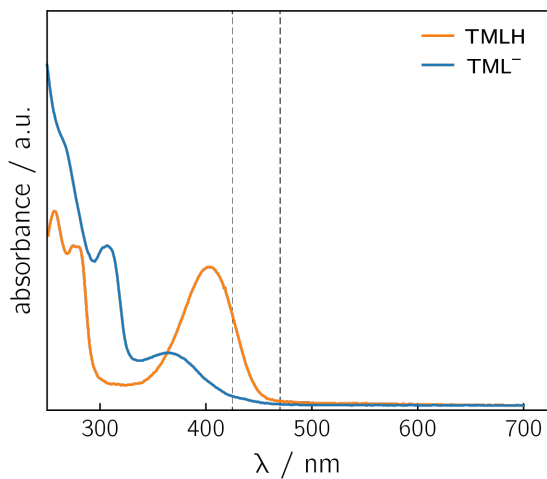
130 Figure 3: UV/vis spectra of TMLH and TML - recorded in water and in 1M NaOH, respectively. The vertical dashed lines indicate the wavelengths chosen for sample irradiation (425 and 470 nm).
