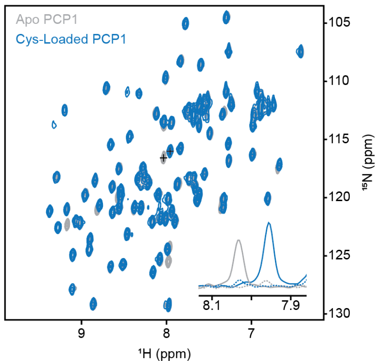
Figure A1. Conformation of loading of PCP1. Loading of PCP1 ( ^{15}\text{N}/^{13}\text{C} ) with the phosphopantetheine analogue was confirmed through 2D HN-HSQC NMR. Upon loading of PCP1, the spectrum of apo PCP1 (grey) shows several characteristic peak shifts that can be used to monitor the chemoenzymatic loading of the prosthetic group (blue) detailed in Sect. 3.2. The inset shows 1D slices of a PCP1 residue that reports on loading (peaks marked with crosses). Solid lines indicate slices at signal maxima and dashed lines indicate slices at the same position when signals are weak or non-existent.
