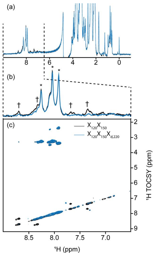
380 Figure 5. Implementation of delayed decoupling into 2D homonuclear TOCSY. X_{150}X_{120} -TOCSY were recorded with (blue) and without (black) a X_{d,220} filter for enhanced suppression of aromatic signals. (a) 1D trace of the detected dimension. The aliphatic region is identical in both spectra but X_d improves the suppression of aromatic signals. (b) Zoom of the spectral region from 6.5 to 9.0 ppm emphasizing the reduction of aromatic signals. Daggers denote aromatic signals from PCP1 that are not suppressed in the TOCSY- X_{120}X_{150} experiment lacking X_d . Asterisks denote signals from the prosthetic that are preserved. (c) Cross peaks between aromatic signals of PCP1 are largely suppressed in the 2D-TOCSY upon addition of our delayed decoupling technique with no loss in signal sensitivity for unlabeled signals.
