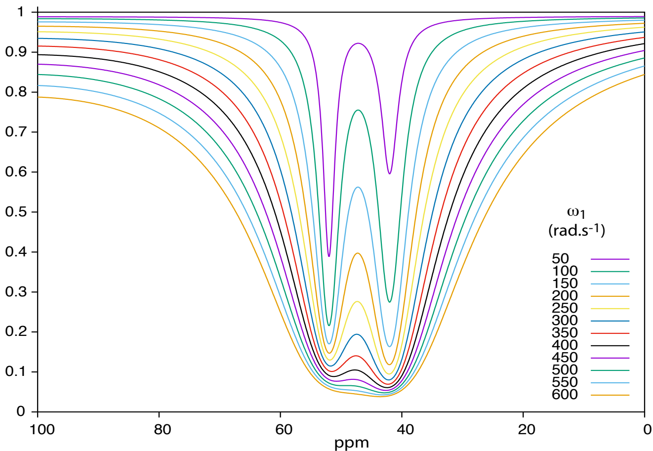
Figure 8. Simulation of ^{129}\text{Xe} Z-spectra at 1 Tesla for a mixture of two cryptophanes according to the saturation field strength. Conditions for the simulation: see text.
