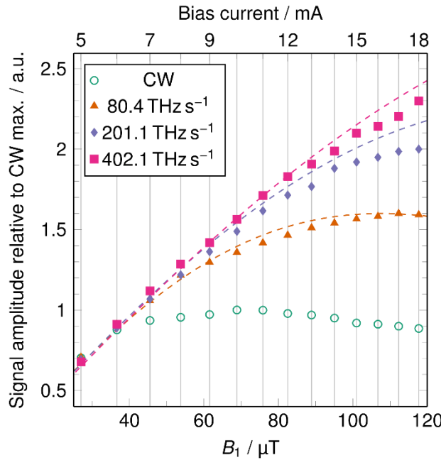
290 Figure 4: Signal amplitudes of CW-EPRoC (○) and transient RS-EPRoC for three scan rates ( 80.4 \text{ THz s}^{-1} , ▲, 201.1 \text{ THz s}^{-1} , ◆, and 402.1 \text{ THz s}^{-1} , ■) as a function of bias current (x-axis, top) and corresponding B_1 magnitudes (x-axis, bottom). The dashed lines are simulations of the RS signals.
