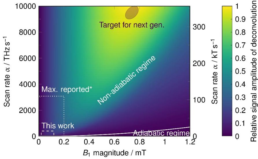
Figure 5: Relative simulated signal amplitude of the deconvolved RS spectrum as a function of both B_1 and scan rate \alpha . The solid line defines the adiabatic and non-adiabatic regions (Eq. (4) and (5)). The relaxation times were set to T_1 = 110 ns and T_2^* = 100 ns. The simulation was performed with a constant RS frequency (200 kHz) and increasing scan width (Eq. (7)). The two outlined rectangular regions (dashes) represent the accessible area for the current work as well as that of a study using field-swept RS-EPR where the maximum scan rate *,3 was reported (Mitchell et al., 2011b). The ellipse shows the target region for the next-gen. EPRoC where the maximum signal is obtained. An improvement of the signal amplitude by a factor of about 5 is expected.
