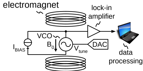
Figure 6. Experimental setup used to obtain the data of Fig. 7. The setup is almost identical to the one in Fig. 1b, with the difference of exchanging the permanent magnet for an electromagnet.
