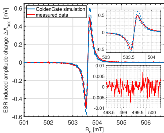
Figure 7. Comparison of the circuit simulator model of section 7 for the ESR induced amplitude shift with measured data of a 14 pl DPPH sample obtained using the VCO prototype presented in Handwerker et al. (2016) used in the setup of Fig. 1b. For comparison, the measured results are referred to the oscillator output by dividing them by the lock-in gain and the demodulation sensitivity of the built-in AM demodulator. Top inset: Zoom-in of the simulated and measured signals. Bottom inset: Zoom-in of the measured signal used for the noise calculation. Measurement conditions: V_{\text{TUNE}} = 2.8 \text{ V} , I_{\text{BIAS}} = 1.7 \text{ mA} , simulated ac current in coil I_{\text{coil,peak}} \approx 8 \text{ mA} corresponding to B_1 \approx 16.8 \mu\text{T} .
