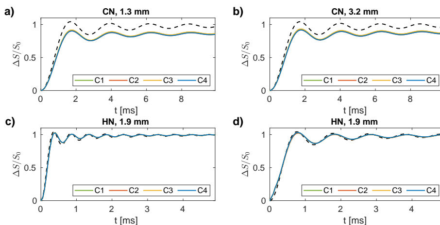
Figure 8. a) / b) Simulated REDOR curves for a CN spin pair with a value of 2 kHz for the anisotropy of the dipolar coupling tensor \frac{\delta I S}{2\pi} at a carbon resonance frequency of 150 MHz in a 1.3 mm MAS probe (a) and a 3.2 mm MAS probe (b) assuming a spinning frequency of 20 kHz. The nominal rf-field strengths were set to 100 kHz (62.5 kHz) for C and 62.5 kHz (50 kHz) for N in the 1.3 mm (3.2 mm) probe. For all four cases C1–C4, the resulting recoupling efficiencies are significantly lower than the theoretical REDOR curve (dashed line). Amplitude modulations (C2 and C4) lead to a further marginal deterioration of the recoupling efficiency. The remaining two cases (C1 and C3) are indistinguishable. c) / d) Simulated REDOR curves for a HN spin pair with a \frac{\delta I S}{2\pi} of 24 kHz at a proton resonance frequency of 600 MHz in a 1.9 mm MAS probe assuming a spinning frequency of 40 kHz. The nominal rf-field strengths were set to 125 kHz for H and 50 kHz for N. A scaling of the effective dipolar coupling is achieved by shifting one pulse (c, delay until first pulse t_1 = 2.5 \mu\text{s} ) or both pulses (d, delay until first pulse t_1 = 16 \mu\text{s} ) per rotor period. No significant deviation of any of the four cases C1–C4 from the theoretical REDOR curves (dashed lines) is observed indicating the robustness of these REDOR implementations towards rf inhomogeneity.
