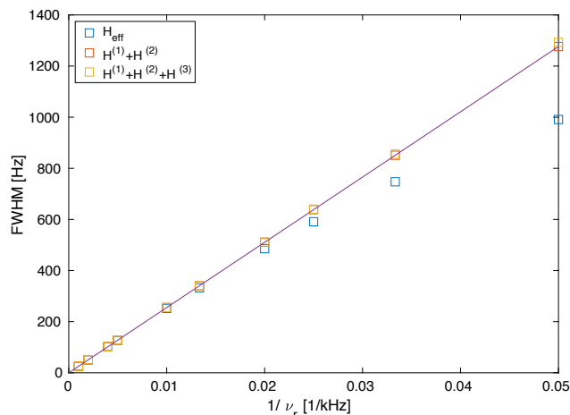
Figure 4. Line width (full-width half max) of a Gaussian line with the same second moment as the powder line shape shown in the SI Fig. S1 ( \text{FWHM} = 2\sqrt{2\ln(2)M_2} ). The line width obtained from second-order and third-order effective Hamiltonian correlates almost perfectly linear with \omega_r^{-1} while the line width obtained from the exact effective Hamiltonian shows some deviations which become more prominent below 50 kHz. This deviation (narrower line width) is the contribution of the fourth-order term as discussed above (see Fig. 3).
