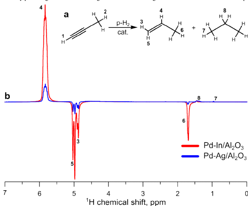
Figure 2: a) Reaction scheme of propyne hydrogenation; b) 1 H NMR ALTADENA spectra acquired during propyne hydrogenation with parahydrogen over Pd-In/Al 2 O 3 (red line) or Pd-Ag/Al 2 O 3 (blue line; the same spectrum as in Fig. 1) catalysts. The reaction temperature was 200 °C, the total gas flow rate was 3.8 mL·s -1 . All spectra were acquired with 8 signal accumulations and are presented on the same vertical scale.
