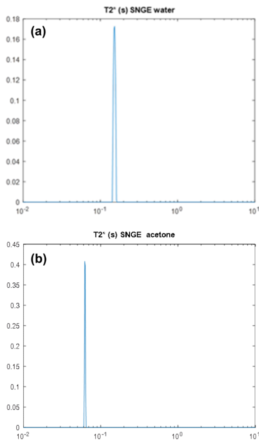
Figure 2. T_2^* distributions obtained from inverse Laplace transform (ILT) (as implemented in MATLAB (MATLAB, 2010) of the data sets measured in the I(+) and I(-) ^1\text{H} SNGE experiments for different delays \Delta . (a) obtained from the ^1\text{H} signal of \text{H}_2\text{O} in 90%:10% \text{H}_2\text{O}:\text{D}_2\text{O} (relaxation constant is about 160 ms), (b) from the ^1\text{H} signal of 90% acetone with 10% acetone- \text{d}_6 (relaxation constant is about 62 ms). \Delta varied from 0 to 70 ms at constant parameters: G_1 = 1.26 \frac{\text{mT}}{\text{m}} , G_2 = 10.7 \frac{\text{mT}}{\text{m}} , \delta_1 = 35 \text{ ms} . Thus, with the ILT analysis, it is possible to extract a distribution of relaxation components f(T_2) . (Berman et al., 2013; Rodin, 2018) In particular, for pure liquids, this distribution f(T_2) showed one relaxation peak. e^{-\Delta/T_2} -Y-scale is an intensity in arbitrary units.
