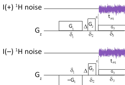
Figure 3. Three-gradient spin noise detected diffusion experiment. The gradient ratios is adjusted according to Eq. (2).
