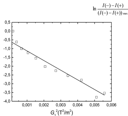
165 Figure 5. G_1^2 -dependence of the normalized difference-spectra integrals of the z-profiles in SNGE I(-) and I(+) diffusion experiments from the three-gradient pulse scheme (Fig. 3) applied to 90%:10% \text{H}_2\text{O}:\text{D}_2\text{O} at T = 295 \text{ K} . The solid line is added for guidance for the eye to emphasize the approximately linear part of the attenuation curve.
