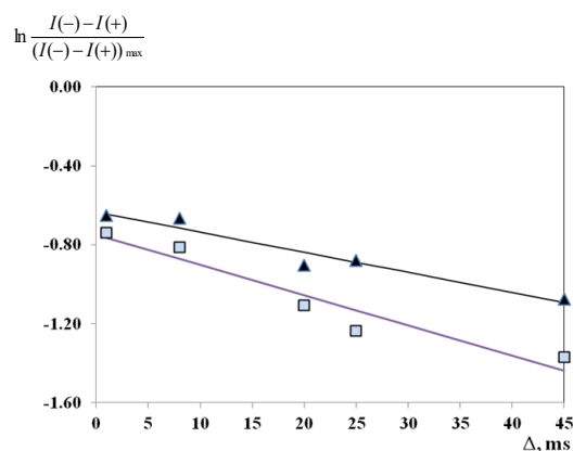
Figure 6. ^1\text{H} SNGE attenuation experiments in a 1:1 acetone-benzene mixture for different delays \Delta between G_1 and G_2 using the three-gradient sequence. (top) data set (triangles) are for the benzene component (chemical shift 7.2 ppm, T_2^* = 91 \text{ ms to } 95 \text{ ms} ), (bottom) data set for the acetone component (chemical shift 2.1 ppm, T_2^* = 60 \text{ ms to } 65 \text{ ms} ) in Fig. S3. \Delta varied from 0 ms to 45 ms at constant parameters of: G_1 = 31.5 \frac{\text{mT}}{\text{m}} , G_2 = 60.1 \frac{\text{mT}}{\text{m}} , G_3 = 1.6 \frac{\text{mT}}{\text{m}}
