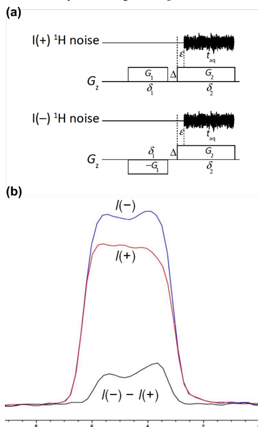
Figure 1: (a) Two-gradient pulse sequence (notably devoid of any RF pulses) used to demonstrate the principle of the spin noise gradient echo (SNGE). The noise blocks of the I(+) and I(-) experiments are stored separately and processed as described elsewhere (Nausner et al., 2009; Pöschko et al., 2017). The power spectra of I(+) and I(-) shown in panel (b) were used to calculate a difference spectrum I(-) - I(+) . Experimental parameters were: G_1 = G_2 = 4 \frac{\text{mT}}{\text{m}} , \delta_1 = \delta_2 = 2 \text{ ms} , \Delta = 0.015 \text{ ms} , \epsilon = 95 0.007 \text{ ms} . 2048 noise blocks were Fourier transformed and their power spectra added for each profile. The line shapes in panel (b) should ideally be rectangular gradient profiles. Deviations are caused by the non-ideality of the gradient system, the finite sample limits and residual radiation damping.
