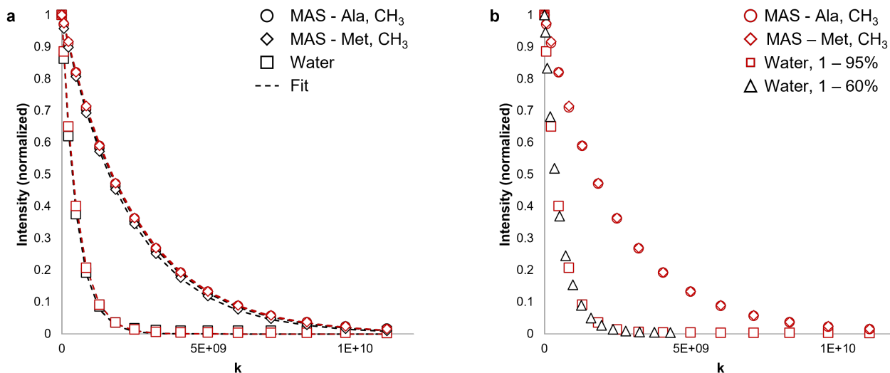
Figure 3. a) Comparison of signal intensity versus the diffusion experiment parameter k = \gamma^2 G^2 \delta^2 (\Delta - (\delta/3) - (\tau/2)) for the alanine and methionine methyl signal of Met-Ala-Ser (MAS, circles, diamonds) and the water signal (squares). Black symbols: the experiment was non-selective; red symbols: selective excitation was used. The dashed lines are the fits to the data using Equation 1. The adjusted R^2 values were all > 0.999 . The diffusion time was \Delta = 250 ms. b) Comparison of signal intensity versus k = \gamma^2 G^2 \delta^2 (\Delta - (\delta/3) - (\tau/2)) for the water (squares, diamonds) and MAS-Ala, Met methyl (circles, diamonds) signals using Sel-BPP-LED. Using the selective experiment, the applied gradient strength experienced by the water signal could be varied independently of the applied gradient strength experienced by MAS. Diamonds: applied gradient strength varied from 1 - 60%. Using the selective excitation experiment, MAS signals were always exposed to an applied gradient varying from 1 - 95%. The experiments were performed in triplicate, the mean values are plotted. The diffusion time was \Delta = 250 ms.
