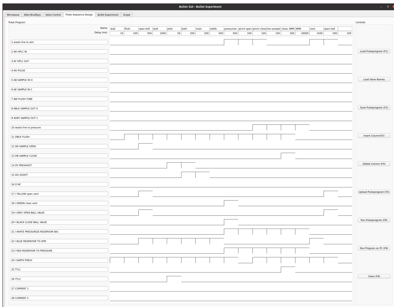
Figure B1. Bullet pulse program for sample ejection, dissolution and injection. The lines 1 to 24 correspond to digital output lines that are connected to pilot valves. The program runs through a sequence of 17 steps. The duration of each step is given in the top row, under its name. Valve 1 connects the outlet of the NMR tube to the atmosphere. Valves 2-9 are not used. Valve 10 connects the output line of the NMR tube to back pressure. Valve 11 applies flush gas on top of the DNP insert, and valves 12 and 13 are used to open and close the ball valve on the DNP insert top, respectively. Valves 14 and 15 apply helium drive gas to the DNP insert via the pilot and main line, respectively, and are used to propel the sample. Valves 17 and 18 open and close a ball valve that is connected to the vent line of the DNP injection device. Valves 19 and 20 open and close the ball valve on the injector. The line above the solvent reservoir can be pressurized with helium (3 bar) using valve 21, or it can be connected to atmosphere using valve 22. Helium pressure can also be applied directly to the solvent reservoir via valve 23. Finally valve 24 controls the pinch valve, which is only opened briefly to inject the sample into the NMR tube. The line TTL1 outputs a TTL signal that triggers the NMR acquisition, the TTL2 signal triggers a scope which measures optical signals and the tunnel current.
