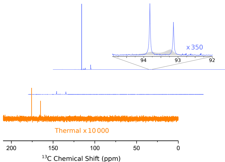
Figure 3. Hyperpolarized ^{13}\text{C} spectra (blue lines) of 1\text{-}^{13}\text{C} pyruvic acid. The middle and upper line show the first two spectra, recorded 1.8 s and 3.8 s after the ejection of the bullet from the polarizer, respectively. The inset shows a magnified view of the doublet near 93 ppm, which is due to the natural abundance carbonyl of pyruvate hydrate. The asymmetry of this doublet yields a ^{13}\text{C} polarization of - 22 % at the (labeled) carboxyl carbon. The full-width at half maximum of both peaks of the doublet is 3.2 Hz. The filled grey area in the inset shows the spectra from our previous publication for comparison (where we used positive DNP leading to an inverted asymmetry). The improvement in resolution is obvious. Note that in our experiment the line near 94 ppm is more intense since we used negative polarization.
