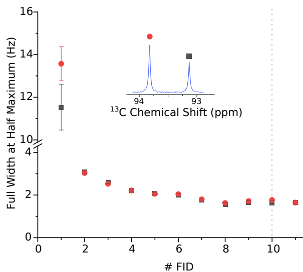
Figure A1. Full width at half maximum of the ^{13}\text{C} doublet due to the carbonyl ^{13}\text{C} atom of pyruvate hydrate. The linewidth of both peaks of > 10 Hz in the first scan is attributed to a gas bubble that rises up the NMR tube during the first scan. The second spectrum, recorded 3.7 s after the sample ejection displays a substantially improved resolution of 3.2 Hz. Over time the resolution improves further, and is better than 2 Hz 14 s after the beginning of the NMR acquisition. Note that there is no significant change in resolution when the back pressure is released 20 s after the beginning of data acquisition (i.e. near the beginning of FID # 10, marked with the dotted line).
