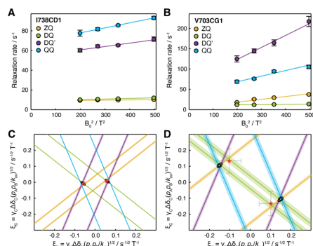
265 Figure 5: Analysis of magnetic field dependence of HE relaxation rates. (A,B) Linear regression analysis of methyl ZQ, DQ, DQ' and QQ HE relaxation rates as a function of B_0^2 , for (A) I738CD1 and (B) V703CG1 resonances. Error bars indicate the standard error determined from curve fitting of relaxation measurements. (C, D) Visualisation of constraints on (\xi_H, \xi_C) parameter space arising from HE measurements. Straight lines indicate values of \xi_H and \xi_C consistent with HE measurements in the upper panels, calculated according to Table 1 assuming fast exchange and subtracting measured CSA contributions. Shading indicates the standard error propagated from linear regression analysis and CSA measurements. Black contours indicate 68 and 95% confidence intervals in \xi_H and \xi_C , based on all four HE measurements and assuming two-state fast exchange. Red symbols indicate \xi_H and \xi_C parameters derived from global fitting of HE and CPMG data (Fig. 6).
