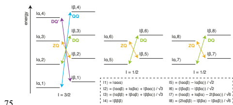
Figure 1: Energy level diagram for an isolated ^{13}\text{CH}_3 spin system. The multiple quantum transitions analysed in this work are indicated with arrows. Energy levels are indexed |\text{C}, \text{H}\rangle according to ^{13}\text{C} and ^1\text{H} spin states, where symmetrised combinations of ^1\text{H} spins are indicated in the inset box (Tugarinov and Kay, 2006).
