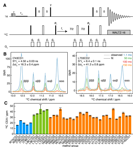
Figure 3: Measurement of methyl ^{13}\text{C} CSA and S_{\text{axis}}^2 \tau_c . (A) ^1\text{H} -coupled HSQC with ^{13}\text{C} Hahn echo. T represents the relaxation time, and the delay \delta = 1/4J = 2 ms. Shaded grey pulses represent consecutive 5 kHz 2 ms \text{H}_x and 3 ms \text{H}_y purge pulses before
