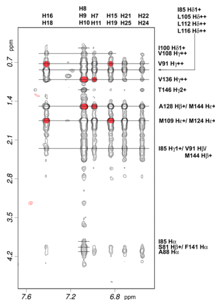
280 Figure 5: Intermolecular NOEs between idoxifene and CaM. A region of the 2D ^{13}\text{C} - ^{15}\text{N} -double-half-filtered NOESY spectrum of the 2:1 idoxifene:CaM complex, processed to exclude the ^{13}\text{C}/^{15}\text{N} bound resonances in the \omega_2 dimension and to include only the ^{13}\text{C} bound resonances in \omega_1 dimension. The ligand resonances corresponding to each strip are marked on the top edge as follows; p -iodophenyl ring (H16/H18), phenyl ring (H8/H9/H10), phenyl ring (H7/H11), p -iodo-phenyl ring (H15/19) and p -phenoxy ring (H21/25 and H22/24). Assignments of the resonances from tr2c are shown on the right. A red circle over the crosspeak indicates examples of NOEs that are violated in the structure calculation corresponding to the data in Fig. S3.
