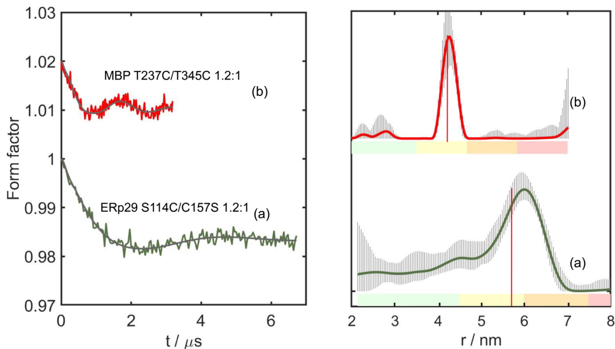
330 Figure 5. DEER distance measurements with DCP-( \beta -Cys) _2 -Gd tags. As in Fig. 4, the left and right panels show the form factors after background subtraction and the distance distribution calculated by DeerAnalysis2018 (Jeschke et al., 2006). All samples were recorded with 1.2:1 Gd^{3+} ion-to-tag ratio. (a) ERp29 S114C/C157S. (b) MBP T237C/T345C. The red vertical lines indicate the maxima of the modelled distance distributions modelled with the program PyParaTools (Fig. S13; Stanton- Cook et al., 2014). The uncertainties in the distance distributions and ranges of alternative distributions are indicated as in Fig. 4. The primary DEER data are shown in Fig. S9 and the distance analysis of (b) by DeerNet (Worswick et al., 2018) in Fig. S10.
