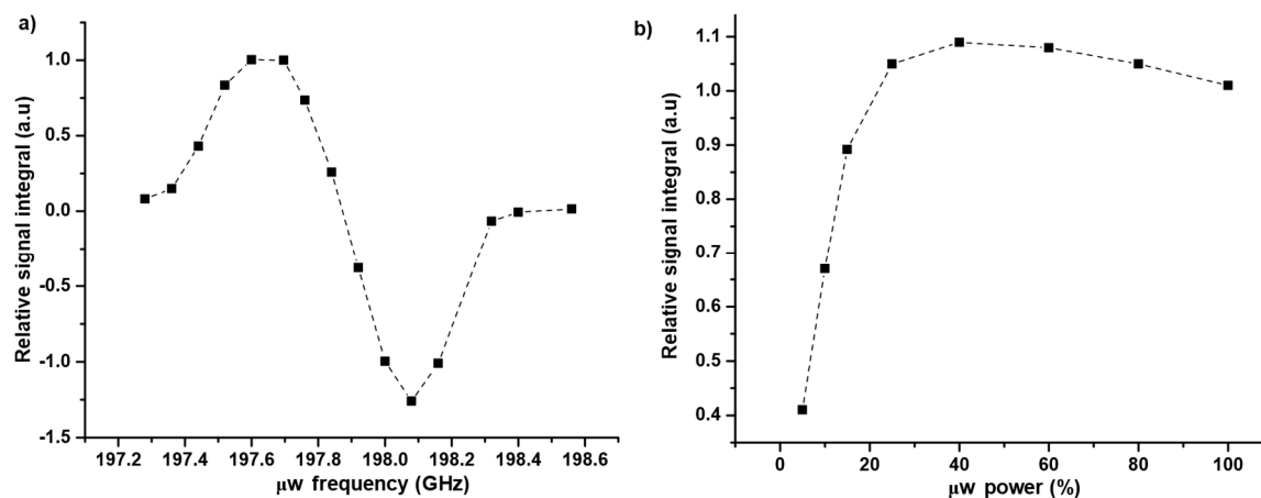
Figure A1. a) Plot of relative ^1\text{H} DNP signal integral vs. \mu w frequency at 50 mM TEMPOL. Signals are normalized with respect to the signal at 197.69 GHz. b) Plot of relative ^1\text{H} DNP signal integral vs. \mu w power (%). Signals are normalized with respect to the signal at 198.08 GHz with a triangular frequency modulation with at bandwidth ( \Delta f_{\mu w} ) of \pm 5 MHz and frequency of 10 kHz.
