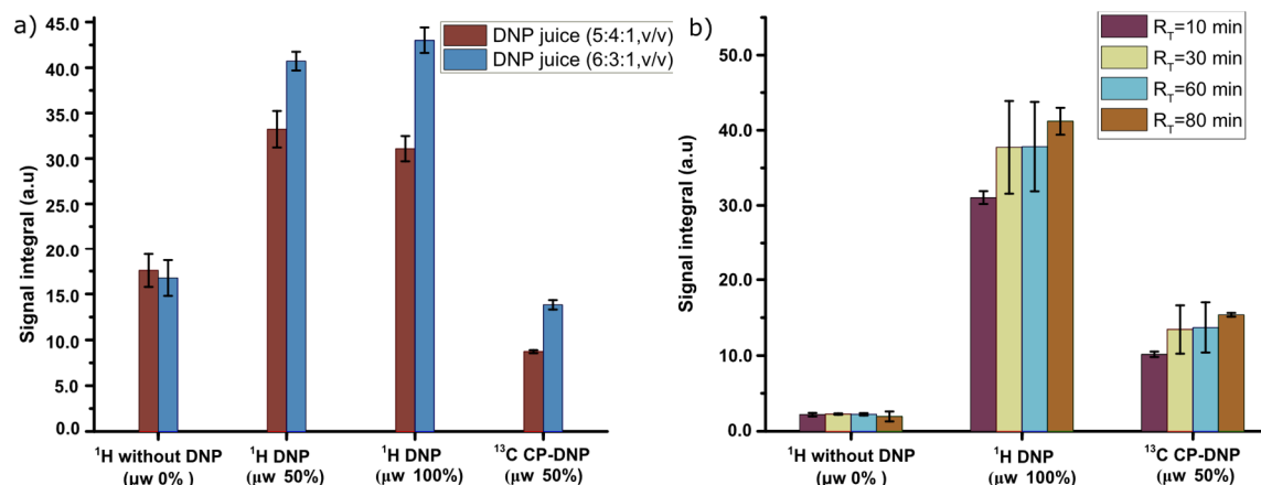
Figure 4. a) Plot of solid-state ^1\text{H} signal without \mu\text{w} as well as ^1\text{H} and ^{13}\text{C} DNP signal integrals at two different DNP juice compositions with 50 mM TEMPOL using optimized \mu\text{w} parameters; b) Plot of solid-state ^1\text{H} and ^{13}\text{C} signal without \mu\text{w} as well as DNP signal integral at different ripening time with same TEMPOL concentration using optimized \mu\text{w} parameters. The standard deviation for every average integral value is calculated from 3 identical samples and displayed as an error bar.
