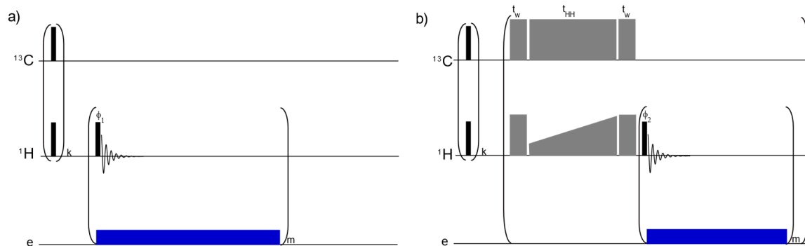
Figure B1. Pulse sequence used to monitor a) ^1\text{H} DNP build-ups and b) solid-state DNP pulse sequence via cross polarization (CP) for d-DNP. A train ( k=64 ) of \pi/2 pulses was applied to both RF channels for pre-saturation. For ^1\text{H} build-up measurements, a small flip angle radiofrequency (RF) pulse is employed after each \mu w irradiation of 10 s (depicted as “blue” block) to monitor the polarization level. Here CP (depicted as “grey” blocks) is performed using adiabatic half passage pulses ( t_w = 175 \mu\text{s} ) to convert longitudinal magnetization into transverse magnetization before the start of the contact pulse ( t_{HH} = 15 \text{ ms} ) and vice versa after the contact. Contact pulses use RF powers of 15 W on ^1\text{H} (using rectangular pulse with constant RF amplitudes of 21 kHz) and 60 W on ^{13}\text{C} (using ramped up pulse with linearly increasing RF amplitudes from 16 kHz to 23.2 kHz). In total, 16 CP contacts ( n=16 ) are made. For each contact, a sequence of m=4 pulses with low-flip-angle pulse ( 5^\circ ) is applied on ^{13}\text{C} channel to monitor the build-up of the
