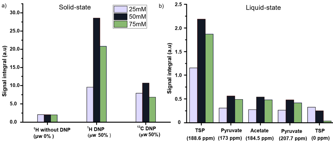
Figure 3. Comparison of signal integral value of a) ^1\text{H} and ^{13}\text{C} signals in the solid-state and b) ^{13}\text{C}\{-^1\text{H}\} liquid-state signal integrals of metabolites with a 25 mM, 50 mM and 75 mM TEMPOL concentration.
