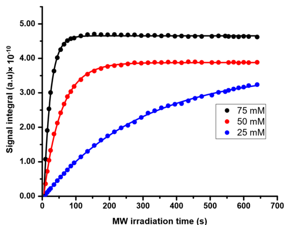
580 Figure C1. ^1\text{H} DNP polarization build up plot at different TEMPOL concentration (75 mM, 50 mM, 25 mM). The data points are fitted monoexponentially to obtain the DNP build-up rate.
