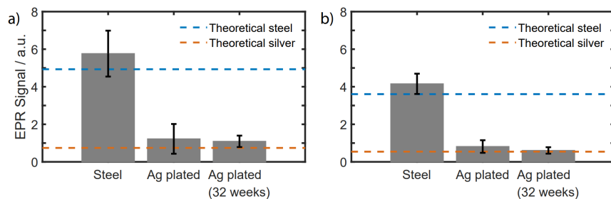
Fig.5: Microwave attenuation before and after plating of (a) 65.5 cm steel waveguide at 197 GHz and (b) 34 cm steel waveguide at 94 GHz. The dotted lines indicate the theoretical attenuation (Zinke, 1990) of a WR28 waveguide made from pure steel or pure silver.
