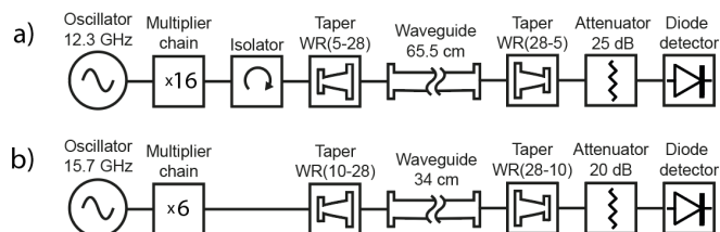
Fig. 2: Schematic setup for measuring transmission losses at (a) 197 GHz and (b) 94 GHz microwave frequency.
