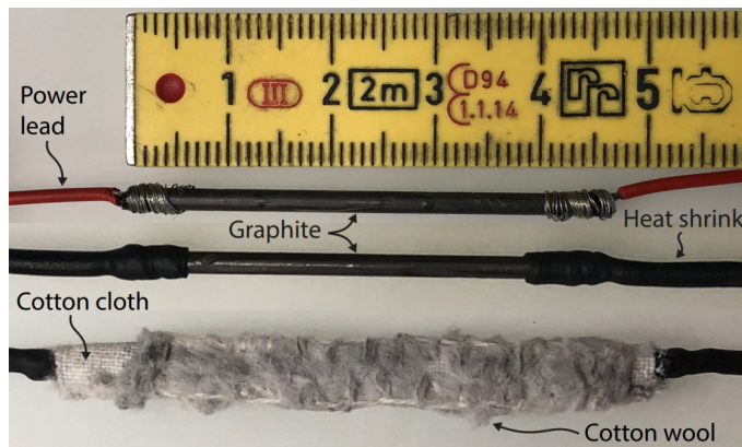
145 Fig.3: Three steps of constructing the plating tool based on pencil graphite as described above. In the bottom, a thin layer of cotton wool is additionally sewn to the fabric for the solution to easily also reach the waveguides inner corners.
