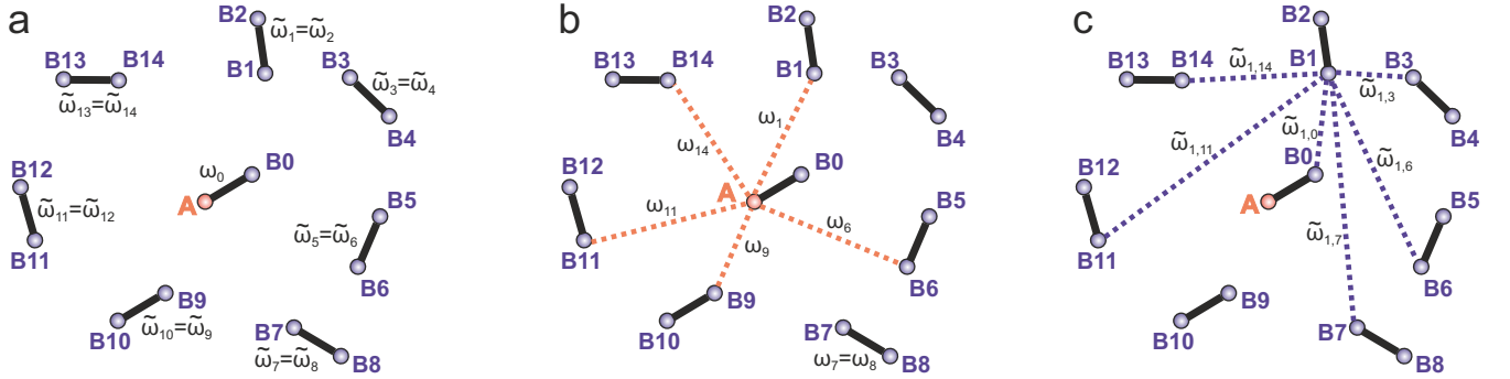
Figure 2. Intra- and inter-molecular electron-electron coupling frequencies for the case of a frozen solution of biradicals. (a) Intramolecular dipolar frequency for the target biradical, containing the A-spin ( \omega_0 ) and the intramolecular dipolar frequencies in other biradicals ( \tilde{\omega}_i ), both spins in these biradicals are B-spins. (b) Intermolecular dipolar frequencies \omega_i describe couplings of A-spin to remote B-spins. (c) The dipolar frequencies \tilde{\omega}_{i,j} describe intermolecular dipolar couplings between B-spins. The case of a frozen solution of monoradicals is obtained by keeping only the intermolecular dipolar frequencies, and dropping the intramolecular ones. Only a selection of intermolecular couplings is shown in the figures to reduce visual crowding.
