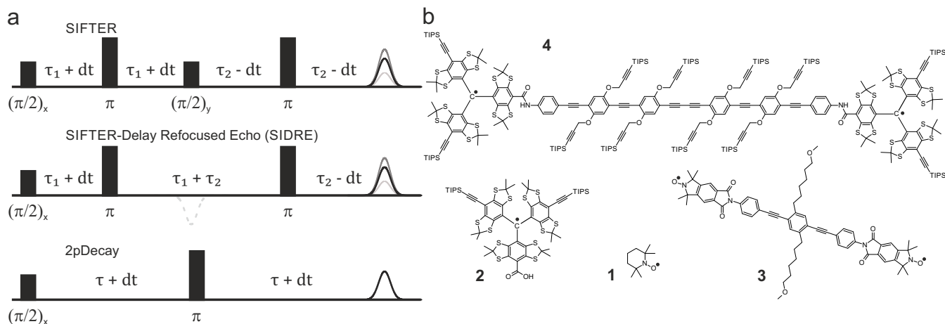
Figure 1. Pulse sequences used in experiments are shown in (a). The time axis in SIFTER traces is t = \tau_1 - \tau_2 , and the interpulse delays are by dt to keep the total transverse evolution time 2\tau_0 = 2(\tau_1 + \tau_2) constant. The chemical structures of the studied compounds are depicted in (b). Nitroxide monoradical (TEMPO) 1 , trityl monoradical 2 , nitroxide biradical 3 , trityl biradical 4 . TIPS is triisopropylsilyl.
