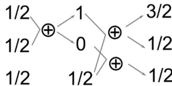
700 Figure 7: Procedure for adding up the angular momenta for the A_3 spin system.
