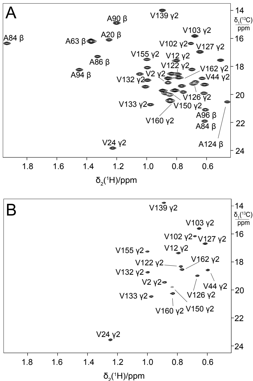
265 Figure 5. Selective ^{13}\text{C} -labelling of the methyl groups of alanine and valine residues in PpiB produced by eCell CFPS. (A) ^{13}\text{C} -HSQC spectrum of PpiB produced from 3\text{-}^{13}\text{C} -pyruvate with valine omitted. Published assignments are shown (BMRB file 11451). The spectrum also displays the cross-peaks of the \gamma_1 -methyl groups, but their assignments have not been reported. Protein yield 2.2 mg, isotope labelling efficiency >75%. (B) ^{13}\text{C} -HSQC spectrum of PpiB produced from 2\text{-}^{13}\text{C} -methyl-acetolactate by eCell CFPS with valine omitted in an eCell CFPS reaction in \text{D}_2\text{O} using deuterated eCells. The ^{13}\text{C} -HSQC spectrum illustrates the selective labelling of the pro- S -methyl groups of valine in a perdeuterated protein. The protein yield was 1.3 mg, and the ^{13}\text{C} -labelling level was 90%.
