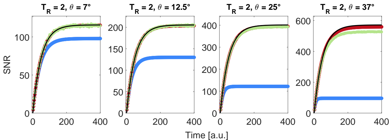
Figure 2. Comparison of noise-free uncorrected (blue), iteratively corrected noise-free (red) and noisy (green) data together with the exponential build-up function (black) given in Eq. 3. Assumed experimental parameters without pulses: P_0 = 0.3 , \tau_{\text{bup}} = 50 , A = 1 , noise = 3.2 \cdot 10^{-4} .
