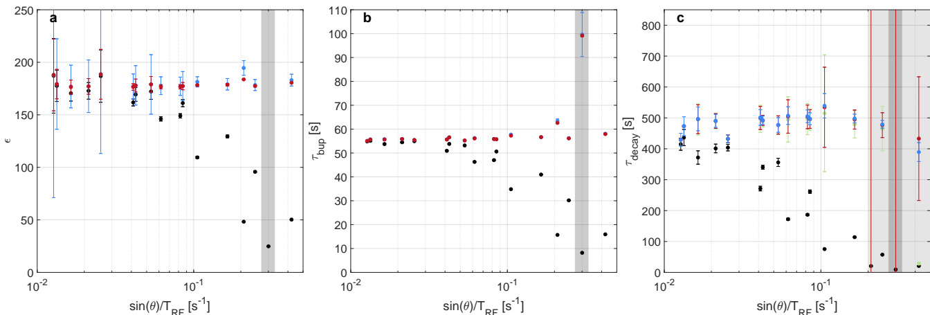
Figure 6. Experimental parameters - enhancement (a) , build-up (b) and decay times (c) - with and without correction for the different experiments with TEMPO in the natural abundance sample as shown in Tab. 3, ordered by the "RF-relaxation-rate" ( \sin(\theta)/T_R ). Black refers to the uncorrected data, red, blue and green to the iterative, CC and 1/\cos^{n-1} correction, respectively. The uncertainties extracted from the 95% fit intervals of the respective build-up and decay measurements are often smaller than the symbol.
