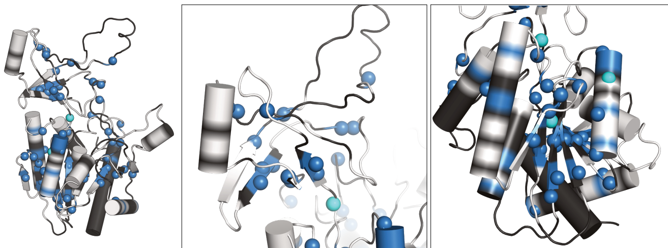
Figure 5. Newly assigned amide hydrogens in TET2 deuterated in \text{H}_2\text{O} shown on its monomeric structure. Amide ^1\text{H} frequencies that were previously inaccessible with perdeuterated samples and that were assigned with the \text{H}_2\text{O}/\text{M9}/\text{lysate} deuteration are represented as spheres on the protein structure. Blue spheres correspond to atoms that could be assigned from the spectra of the \text{H}_2\text{O}/\text{M9}/\text{lysate} -deuterated sample (600 MHz ^1\text{H} Larmor frequency, 55 kHz MAS), while cyan spheres are for atoms that only showed signal in the spectra of the fully protonated sample (950 MHz ^1\text{H} Larmor frequency, 100 kHz MAS). Parts for which the backbone is shown in white regions correspond to those for which heavy-atom assignments have previously been reported Gauto et al. (2019a) ( Gauto et al., 2019a ), while black regions indicate parts with missing heavy-atom assignment. In those parts we did not attempt to get new amide assignments, as the de novo assignment of the backbone would likely require more 3D data sets. Taken together, this data highlights the possibility of detecting amide hydrogens of water-inaccessible regions in the protein. Note that the protein forms a dodecamer (Fig. 4Aa), and for better visibility only the monomeric subunit is shown.
