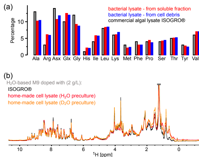
Figure 2. Comparison of the amino-acid composition in a home-made bacterial extract with the one in ISOGR0®. (Aa) The amino acid composition of ISOGR0®, as provided by the manufacturer, is shown as grey bars; the values represent the percentage (weight) of each amino acid in the powder. Data of the home-made preparation from bacterial perdeuterated cultures are shown in blue and red. The preparation made from the soluble-proteins fraction, i.e. contaminant proteins from a protein purification, is shown in red. The preparation made from the insoluble fraction after cell lysis is shown in blue. Asn and Gln are indistinguishable from Asp and Glu with this method. Cys and Trp are destroyed during the processing steps of the analysis. (Bb) 1D 1 H spectra of ubiquitin deuterated in H 2 O based medium supplemented with either commercial algal lysate (black) or the home-made lysate, prepared from the contaminant proteins. The precultures have been made either in H 2 O or D 2 O, as indicated. The similarity of the spectra confirms that commercial algal lysates and bacterial lysates produce similar labelling patterns, as expected from the very similar distribution of amino acids shown in panel (Aa).
