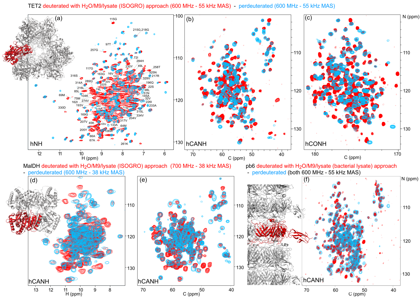
Figure 4. Deuteration in H 2 O enhanced by amino-acid mixtures from cell lysates allows detection of non-exchangeable amide hydrogens. Overlay of (Aa) hNH, (Bb) hCANH, (Cc) hCONH TET2 spectra, (Dd) H-N and (Ee) CA-N projections of the hCANH MalDH spectra, and (Ff) hCANH pb6 spectra. (For the latter, the in-house made bacterial cell lysate was used.) Spectra of samples deuterated by the H 2 O/M9/lysate approach are shown in red, while spectra from perdeuterated samples are shown in blue. All samples were 13 C and 15 N labelled. Peaks that appear to only be present in the perdeuterated sample spectra can be explained by (i) different apparent frequencies of aliased peaks (since the spectral widths and carriers are not identical in the overlaid spectra), (ii) chemical shift perturbations due to small sample-temperature differences, and (iii) different signal/noise ratios of individual peaks.
