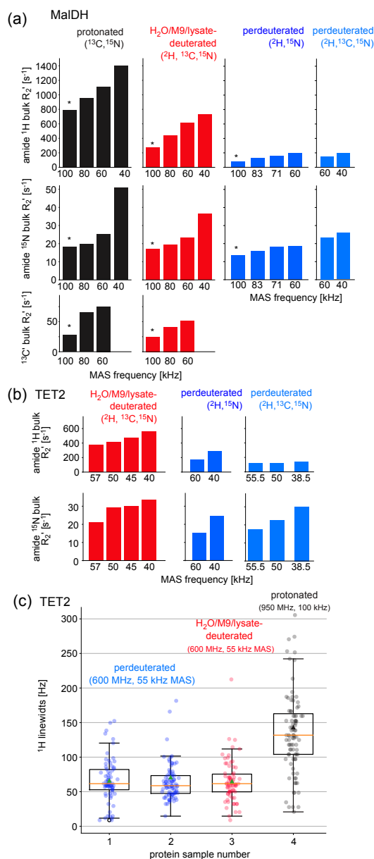
Figure 3. Investigation of coherence life times and line widths in differently labelled samples of two proteins. (Aa) Fitted R_2' decay rate constants for four differently labelled samples of MalDH as indicated. The decay curves for representative experiments, indicated with an asterisk, are shown in Figure A1. All data were recorded at a B_0 field strength corresponding to 700 MHz ^1\text{H} Larmor frequency in a 0.7 mm probe. (Bb) Similar data for the TET2 protein. (Cc) ^1\text{H} line widths of TET2 in deuterated samples produced in \text{D}_2\text{O} -based M9 medium (blue), produced in \text{H}_2\text{O} -based M9 medium doped with 2 g/L deuterated algal extract (red) or fully protonated (black). Spectra are shown in Fig. A2.
