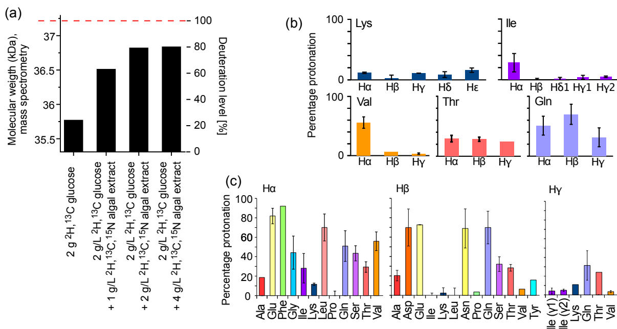
Figure 1. Deuteration using H 2 O-based medium doped with algal lysate. (Aa) Deuteration level of I. islandicus MalDH (33.55 kDa) expressed in H 2 O with either ^2\text{H}, ^{13}\text{C} glucose only (2 g per liter of culture) and ^{15}\text{N} , or with additional use of ^2\text{H}, ^{13}\text{C}, ^{15}\text{N} algal extract (ISOGRO®) at three different concentrations (1, 2, 4 g per liter of culture). The reported molecular-weight values are from intact mass spectrometry. The dashed red line indicates the theoretical molecular weight of fully deuterated MalDH (assuming all exchangeable hydrogens are ^1\text{H} ). (Bb, Cc) Residual protonation level for aliphatic sites, determined by solution-state NMR of a sample of ubiquitin produced in H 2 O-based M9 medium supplemented with ^2\text{H}, ^{13}\text{C}, ^{15}\text{N} algal extract (2 g/L). Amino acid types missing in this plot are either not present in ubiquitin, excluding the possibility for quantification (Trp) or are not visible or unresolved (Met, His, Arg).
