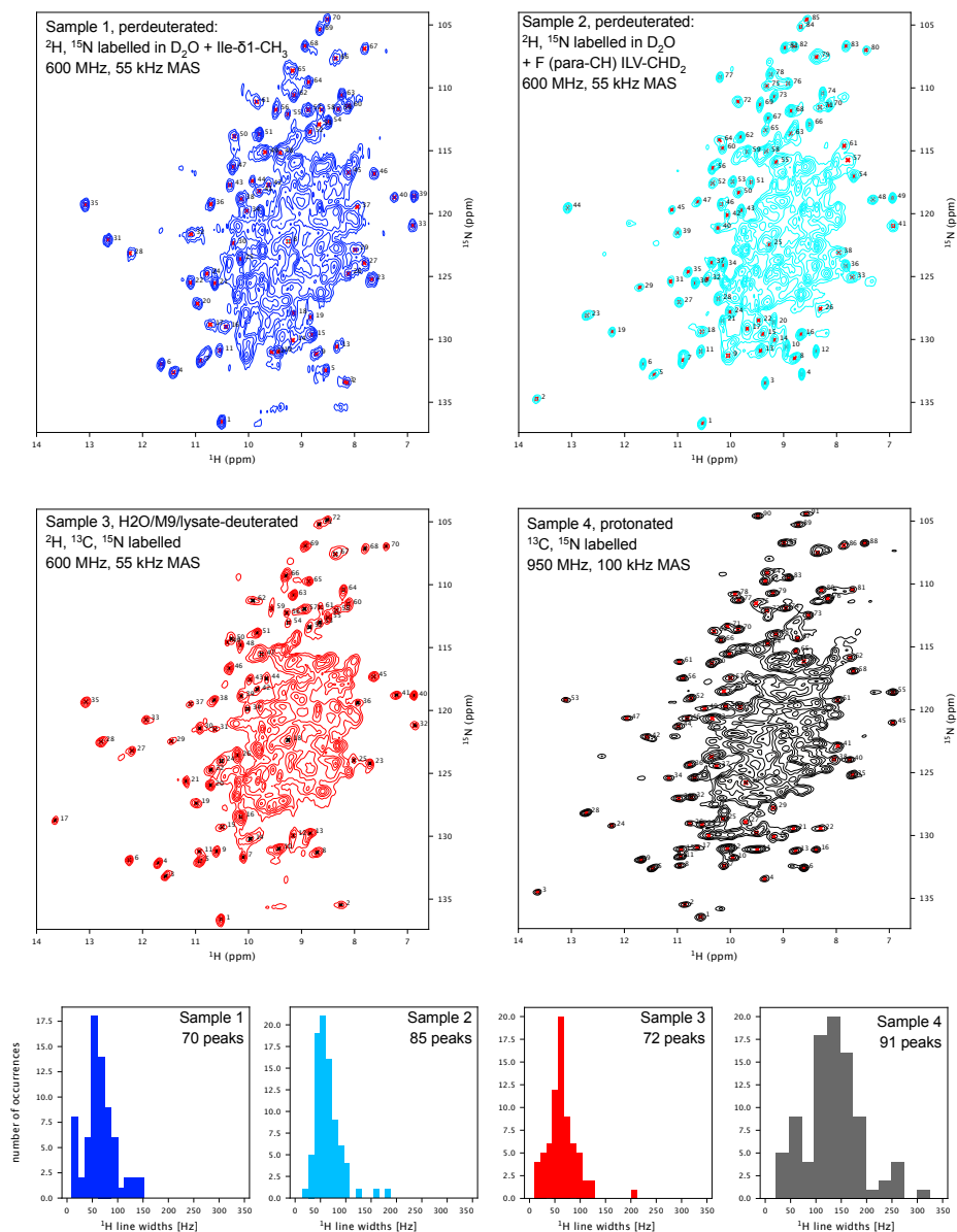
Figure A2. Line widths in differently labelled samples. These spectra have been used to extract the ^1\text{H} line width statistics reported in Figure 3Cc. Samples 1 and 2 were deuterated in a D 2 O based culture; they have been used for previous studies Kurauskas et al. (2016) ; Gauto et al. (2019a) ( Kurauskas et al., 2016 ; Gauto et al., 2019a ), for which additional labelling has been used as indicated. Note that this labelling introduces protons only at the terminal methyl of Ile (sample 1) or a single hydrogen at the terminal methyls of Ile, Leu, Val and the \zeta -position of Phe (sample 2), far from the amide sites, and does not lead to significant changes of amide ^1\text{H} line widths. Sample 3 has been deuterated in H 2 O based medium supplemented with deuterated ISOGRO ® . Sample 4 is fully protonated; note that the latter has been measured at 950 MHz ^1\text{H} Larmor frequency, while all other spectra were measured at 600 MHz. Crosses indicate the peaks that have been used for the analysis, and the plots at the bottom indicate the binned line width distribution.
