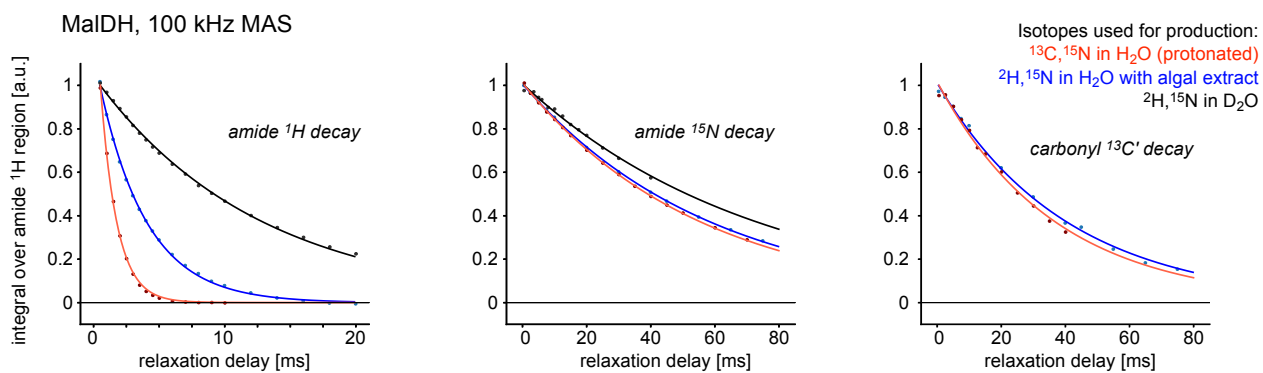
Figure A1. Examples of coherence decays in differently labelled samples. The decay curves correspond to the data marked with an asterisk in Figure 3Aa. The solid lines are fits to the data, using a mono-exponential decay function. The data have been normalised such that the fitted curve at a relaxation delay of zero is at unity.
