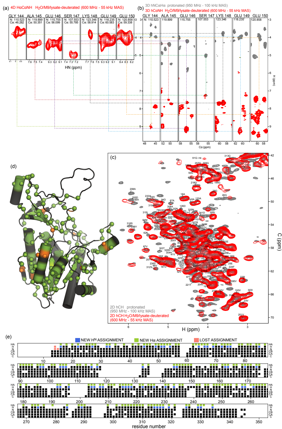
Figure 6. Protein deuteration in \text{H}_2\text{O} allows assignment of \text{H}\alpha hydrogens
