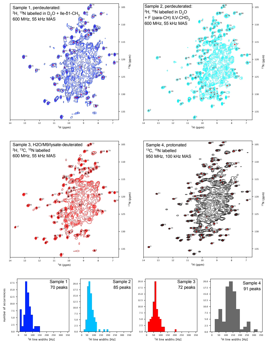
Figure A2. Line widths in differently labelled samples. These spectra have been used to extract the ^1\text{H} line width statistics reported in Figure 3C. Samples 1 and 2 were deuterated in a \text{D}_2\text{O} based culture; they have been used for previous studies Kurauskas et al. (2016); Gauto et al. (2019a), for which additional labelling has been used as indicated. Note that this labelling introduces protons only at the terminal methyl of Ile (sample 1) or a single hydrogen at the terminal methyls of Ile, Leu, Val and the \zeta -position of Phe (sample 2), far from the amide sites, and does not lead to significant changes of amide ^1\text{H} line widths. Sample 3 has been deuterated in \text{H}_2\text{O} based medium supplemented with deuterated ISOGRO ® . Sample 4 is fully protonated; note that the latter has been measured at 950 MHz ^1\text{H} Larmor frequency, while all other spectra were measured at 600 MHz. Crosses indicate the peaks that have been used for the analysis, and the plots at the bottom indicate the binned line width distribution.
