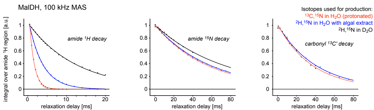
Figure A1. Examples of coherence decays in differently labelled samples. The decay curves correspond to the data marked with an asterisk in Figure 3A. The solid lines are fits to the data, using a mono-exponential decay function. The data have been normalised such that the fitted curve at a relaxation delay of zero is at unity.
