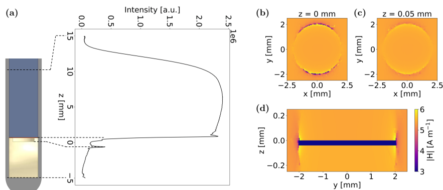
Figure 4. (a) Frequency encoded ^1\text{H} density profile of the experimental setup with horizontally placed Cu foil. (b) – (c) B_1 field intensities in layers exactly on top of the Cu disc and 50\ \mu\text{m} above it, respectively. (d) B_1 field intensities in the sectional side view through the Cu disc.
