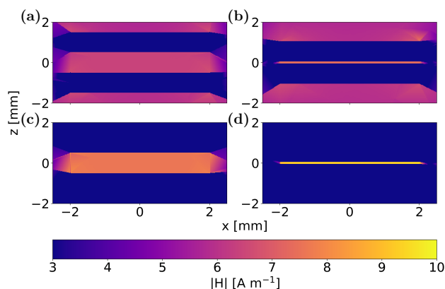
Figure 5. Spatial distribution of calculated B_1 field in a central sectional plane perpendicular to the coin surface with coins of (a) 1 mm distance and 1 mm thickness, (b) 0.1 mm distance and 1 mm thickness, (c) 1 mm distance and 5 mm thickness, (d) 0.1 mm distance and 5 mm thickness. The origin of the z -axis is centred between the two coins.
