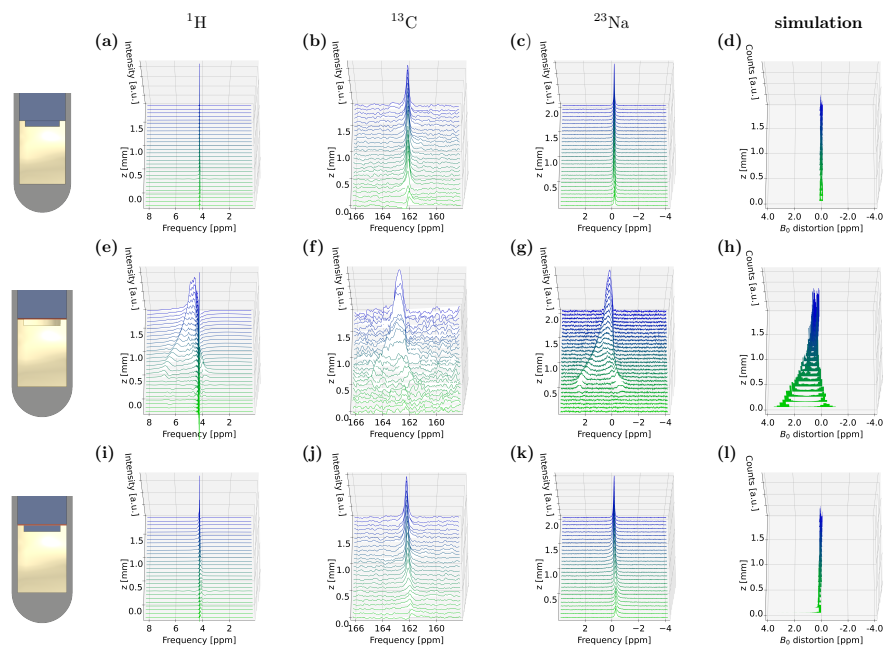
Figure 3. Spatially resolved NMR spectra of CSI measurements of experimental setups (a) – (c) without Cu foil, (e) – (g) with Cu foil and air underneath and (i) – (k) with Cu foil and electrolyte underneath, depicted between z = [0, 2] mm. Spectra are shown for ^1\text{H} , ^{13}\text{C} and ^{23}\text{Na} , respectively. Simulated B_0 distortions, represented by histograms over the same z interval, for the case of (d) no Cu foil and water filled notch, (h) air and (l) water underneath the Cu foil, respectively. The histograms were corrected under the assumption of perfect shimming of the sample without Cu foil.
