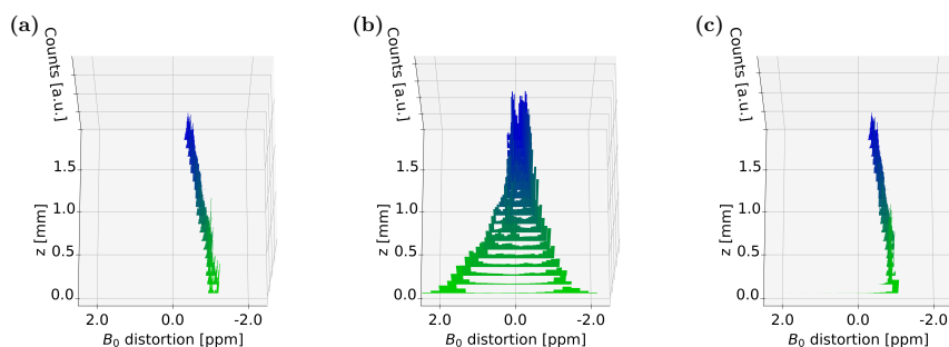
Figure A1. Simulated B_0 distortions, represented by histograms over the z -axis, for the case of (a) no Cu foil and electrolyte-filled notch, (b) air and (c) electrolyte underneath the Cu foil, respectively. The histograms were not corrected in terms of shimming.
